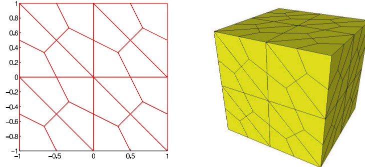
Fig. 5. Test meshed cavities in 2D and 3D
