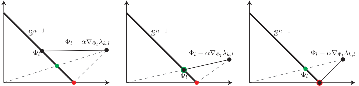
FIG. 3.2. Behavior of the projection operators. The black dots represent \Phi_l and \Phi_l - \alpha \nabla_{\Phi_l} \lambda_{k,l} as labeled. The red ones are the orthogonal projection of \Phi_l - \alpha \nabla_{\Phi_l} \lambda_{k,l} , the green ones its simple projection. Simple projection has a lesser tendency to “send” the functions \Phi_l towards the vertices of \mathbb{S}^{n-1} .
