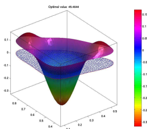
Figure 4: \lambda_2^{cd}
