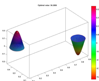
Figure 3: \lambda_1^{cd}
