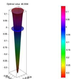
Figure 5: \lambda_3^{cd}
