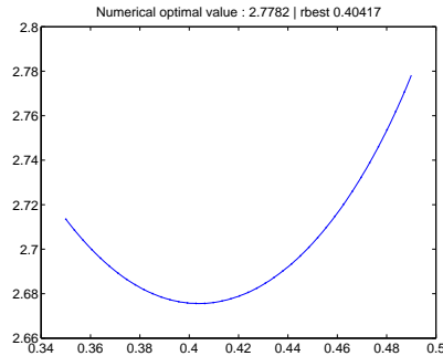
Figure 4: Numerical evaluations of the shape functional w.r.t. the width ( d(\Omega) = 1 )
