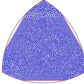
Figure 1: A cutted Reuleaux triangle
