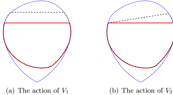
Figure 3: Linear vector fields
