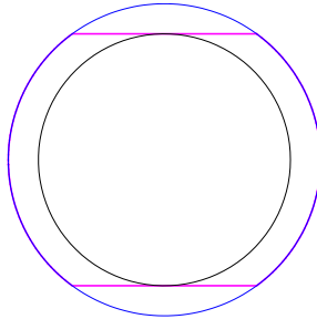
Figure 2: Optimal set when the maximal inscribed ball is not unique
