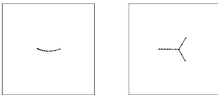
FIGURE 10. Optimal sets of length 0.5 and 1 in a unit square
