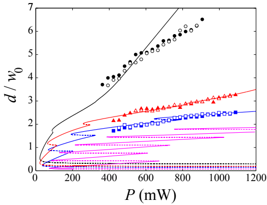
FIG. 2: (Color online) Power dependence of the liquid fiber diameter for beam waists w_0 = 1.8 \mu\text{m} (black line and circles), 2.7 \mu\text{m} (red line and triangles), 3.5 \mu\text{m} (blue line and squares) and 7.0 \mu\text{m} (magenta). Filled and open symbols refer to increasing and decreasing power, respectively. Solid and dashed lines corresponds respectively to stable and unstable states predicted by the model.
