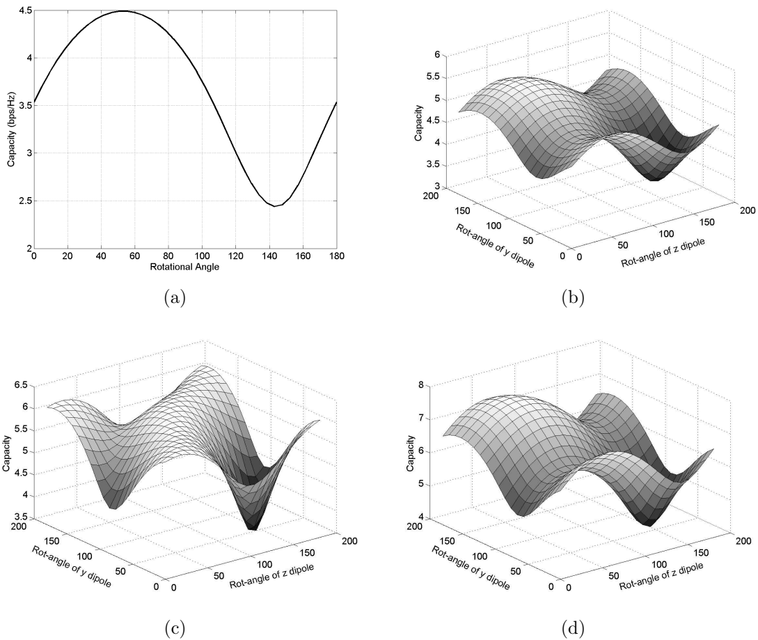
Figure 1.20: Performances of (a) 1 \times 1 SISO, (b) 1 \times 2 SIMO, (c) 2 \times 2 MIMO as the same antenna position, (d) 2 \times 2 MIMO as the separated antenna position while the receiving antenna is rotating on plane y-z
