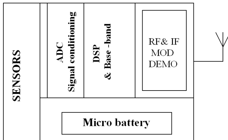
Figure 1.21: Typical wireless sensor node
