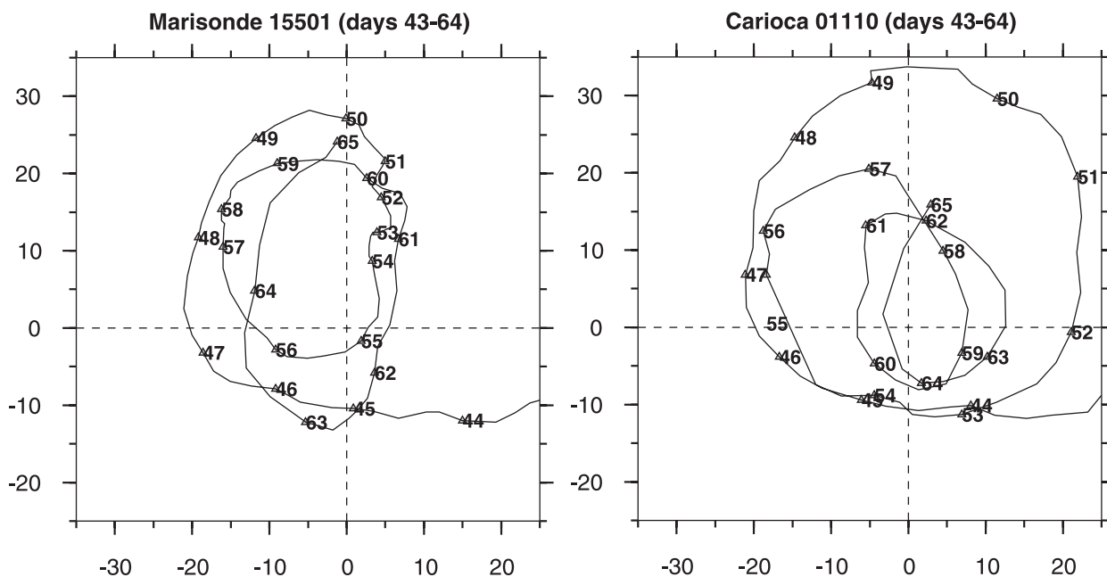
FIG. 9. Trajectories in February and early March of two surface drifters (Marisonde 15501 and Carioca 01110) in relative position to the SCV center (based on Surdrift 24331 GPS position data). The 2001 calendar day is reported at the float position at the beginning of each day.
