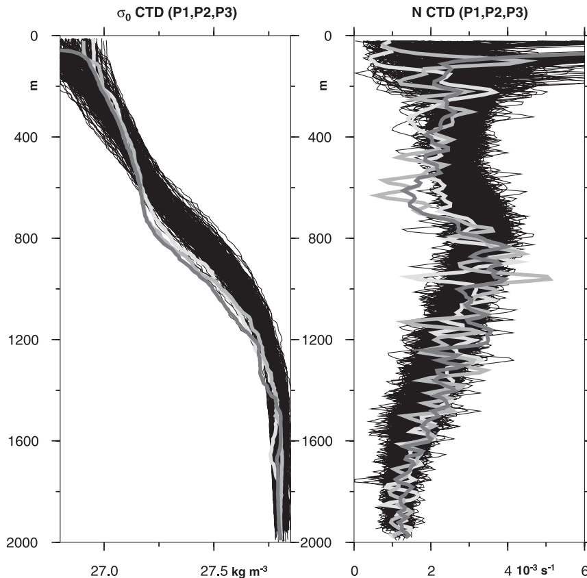
FIG. 6. As in Fig. 5, but for the vertical profiles of \sigma_0 and Brunt–Väisälä frequency N .
