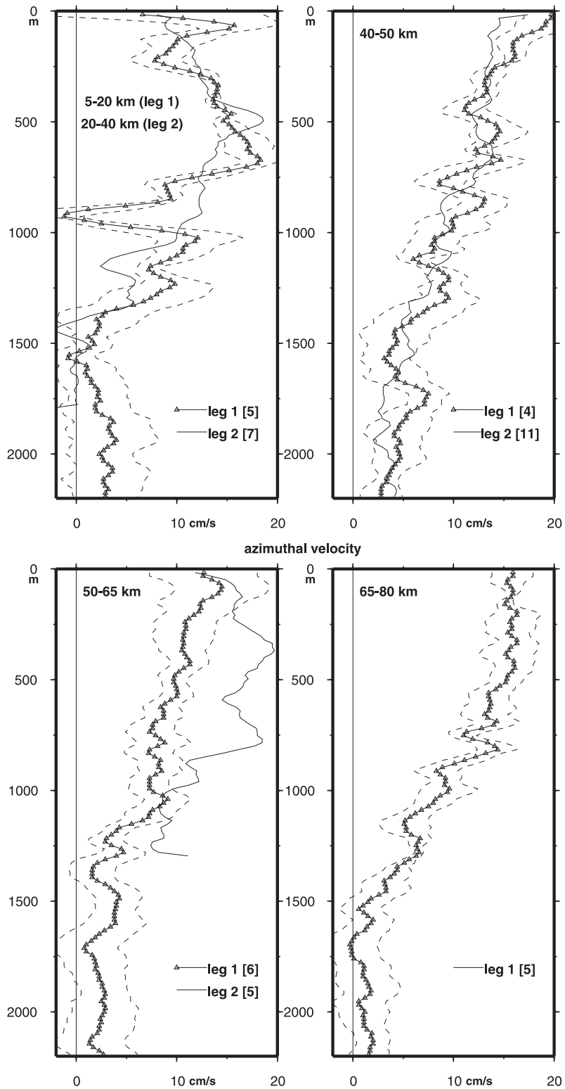
FIG. 10. Average profiles of azimuthal velocity from LADCP profiles as a function of depth for different radius ranges. The leg 1 averages are indicated (triangles) as well as a 2\sigma uncertainty range (dashed curves). The full curve is for the leg 2 average. The number of LADCP stations is indicated in the brackets.
