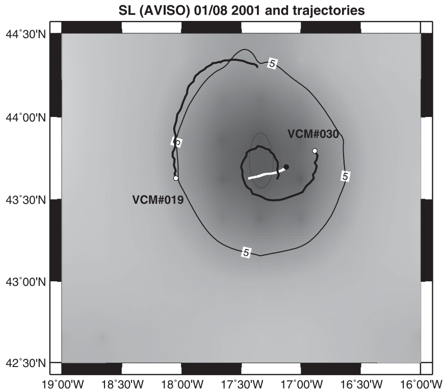
FIG. 12. Sea level (cm) from satellite altimetry (AVISO product) over eddy A1 on 1 Aug 2001 (contours 0, 5, and 10 cm). Here, 10-day portions of the SCV center trajectory (white) as well as floats VCM 030 and VCM 019 (black). Dots plotted at beginning of each trajectory.
