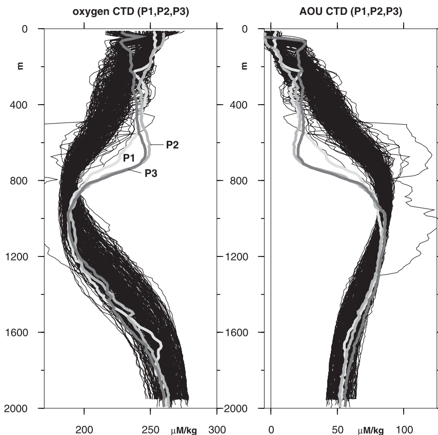
FIG. 5. Vertical profiles of dissolved oxygen ( \mu\text{M kg}^{-1} ) as a function of pressure from 0 to 2000 dbars for all CTD casts ( >80 ) taken during leg 1 of P1 (February), P2 (April), and P3 (September) in 2001. Also CTD casts 23 (leg1, P1), 41 (leg1, P2), 26 (leg 1, P3) collected in the SCV core (close to VCM 030 and MV 19954).
