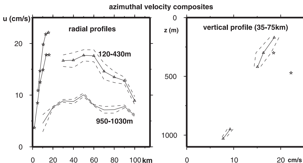
FIG. 13. Azimuthal velocity as a function of distance to eddy (left) center or (right) depth. All velocity data from the floats and from the current meters within the eddy have been included, except for the two floats within the SCV (MV 19954 near 450–500 m and VCM 030 near 250–300 m), which are treated separately (stars; right corresponds to maxima of left). First, azimuthal velocity relative to the smoothed eddy center position (see Fig. A1) is estimated. Then, the inertial and high-frequency oscillations are filtered out, and resulting velocities are averaged in 10-km radius bins and in depth ranges. Profiles are continuous from at least 35 km for data in 5 depth ranges: one between 120 and 2020 m, the others near 300, 420, 950, and 1030 m. (left) The three upper profiles (two lower profiles) are averaged together (solid line), and an error on this average ( 2\sigma range between the dashed lines) is estimated based on the deviations with respect to the average profile normalized by a vertical dependency (see right panel). (right) An average depth profile by averaging bins between 35- and 75-km radius range [an error on this average is estimated based on the deviation of individual radius bins from an average profile (from left panel); 2\sigma range between the dashed lines].
