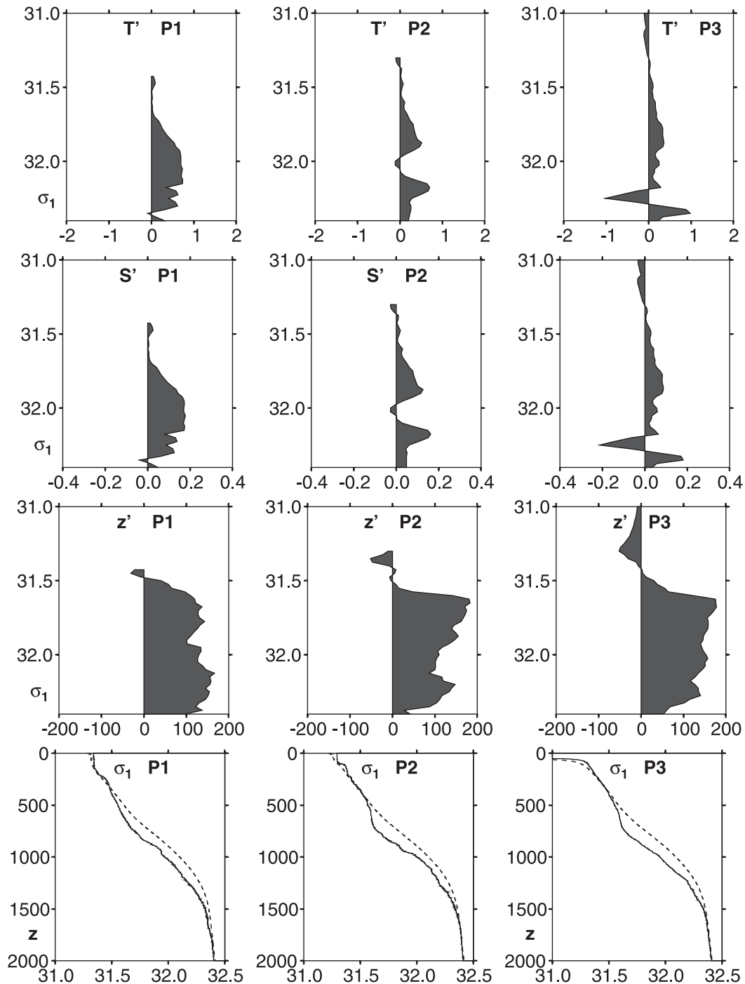
FIG. 7. Temperature, salinity, and depth anomalies of isopycnals in a \sigma_1 (potential density referred to 1000 dbar) coordinate for stations in the core. The anomalies are estimated with respect to an average profile (in \sigma_1 coordinates) of all stations in the POMME domain within 200 km north or south of the eddy core. (bottom) The \sigma_1 profiles of the core station (solid line) relative to mean profile of nearby stations (dashed line) as a function of depth.
