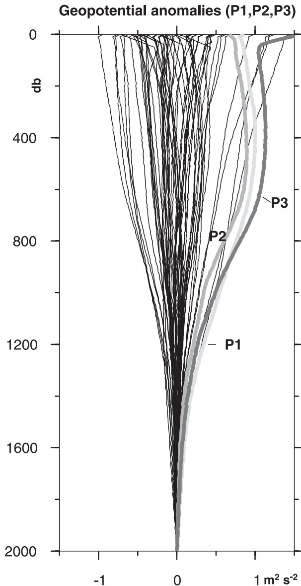
FIG. 14. Vertical profiles of GPA relative to 2000 dbar calculated from all the CTD casts of P1 leg 1 (R/V Atalante ) are represented (solid lines) and overlaid with the core profiles (thick line) for P1 CTD cast 23 (light gray), P2 CTD cast 41 (gray) and P3 CTD cast 26 (dark gray).
