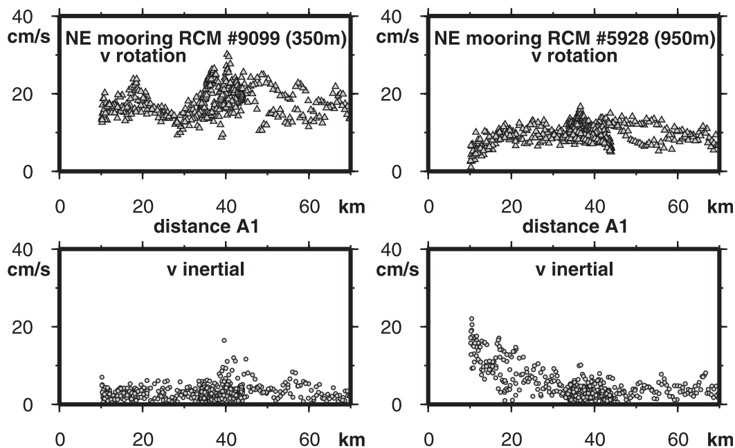
FIG. 11. Estimates every 8 h of (bottom) near-inertial velocity amplitude and (top) averaged azimuthal velocity (upper panels) as a function of distance to eddy center from 2 current meters on northeast mooring (left, 350 m; right, 950 m). The hourly velocities are first calculated relative to a moving referential origin: for distances less than 20–25 km, this is the position of the SCV center; for larger distances, the smoothed eddy center position is retained (Fig. A1). Over 17-h time series segments, the relative velocities are fitted to the sum of a mean and an inertial oscillation to estimate a near-inertial velocity amplitude. The mean is then decomposed in azimuthal and radial velocity components.
