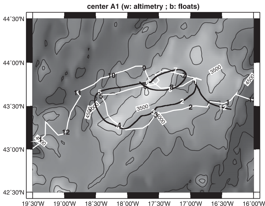
FIG. A1. The A1 eddy center position from November 2000 to September 2001 superimposed on bottom topography (lighter for shallower depths). The month (number) is reported on the curve at each beginning of month. White curve: based on weekly altimetry maps; black curve: a smoothed version of SCV position of Fig. 1.
