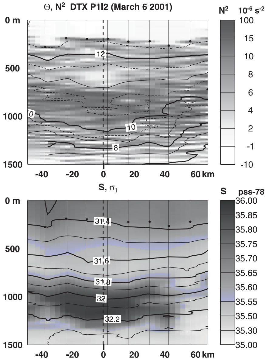
FIG. 4. Zonal sections from XCTDs launched by the R/V d'Entrecasteaux cutting the eddy, less than 2 km north of its center on 6 Mar. The horizontal axis is zonal distance from the eddy center (indicated by a vertical dashed line), and vertical lines indicate where XCTDs were launched. The dots indicate the depth of mixed layer (based on a SST - 0.1°C criterion). The section was done during and after a large wind event and when the surface density was the highest based on drifter data. (top) Potential temperature (lines) with Brunt-Väisälä frequency (grayscale) and (bottom) potential density \sigma_1 (with 1000-dbar reference level) and salinity (grayscale).
