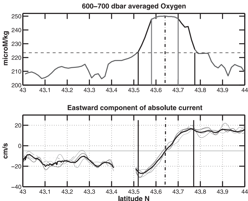
FIG. 3. The 30 Apr 2001 R/V Atalante meridional section west of the eddy center. (top) Average oxygen in the 600–700-dbar layer in which the oxygen maximum is found. (bottom) Zonal velocity from the ship VM ADCP at different depths (the thick line is for the average, 445–621 m). The vertical lines indicate roughly the position closest to eddy core (mixed line): (top) the edge of the homogeneous core, and (bottom) the location of the velocity maxima. Notice that the center of the SCV seems to correspond to a westward zonal velocity of -4 \text{ cm s}^{-1} (horizontal line in bottom panel), in accordance with the translation estimates of the core at that date based on the floats.
