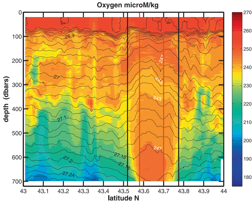
FIG. 2. The 30 April north–south tow-yo CTD section of the R/V Atalante passing some 5–6 km to the west of the SCV center at 43.64°N (profiles every 1 km). The plot is for potential density (contours) and oxygen ( \mu\text{M kg}^{-1} ; color). The red lines indicate roughly the eddy core boundaries, and the black line is the limit of the intermediate region.
