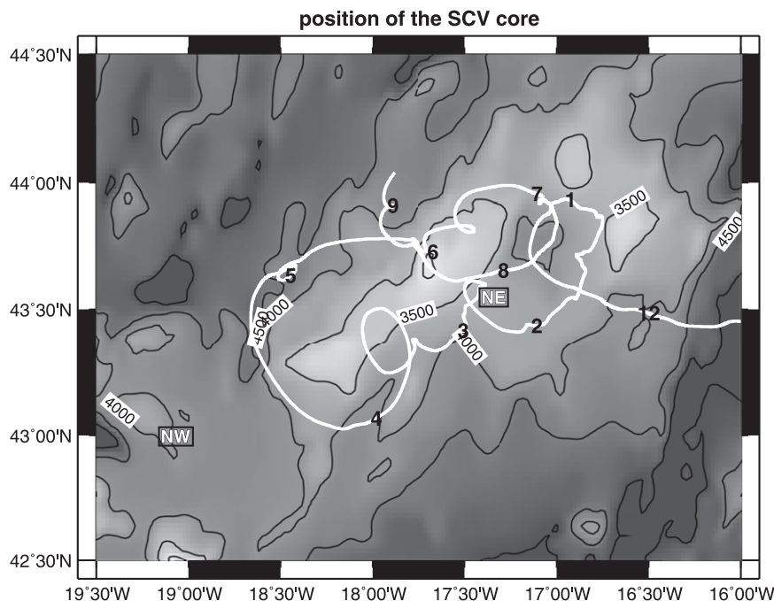
FIG. 1. SCV center position (white line) from November 2000 until September 2001 superimposed on bottom topography (light above 3500 m, which corresponds to a segment of the Azores–Biscay ridge). The month number (in black) is reported on the curve at beginning of each month. Two current meter moorings locations are indicated (NE and NW). See text for explanations on how the SCV center position is estimated from two float trajectories.
