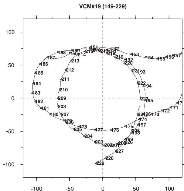
FIG. 15. Two-month trajectories for float VCM 19 in relative positions to smoothed eddy center position (Fig. A1). During that time (2001 calendar days 149–229), the eddy center turns anticyclonically around 44°N, 17.5°W (Fig. 1). The calendar day is reported at the float position at the beginning of each day.
