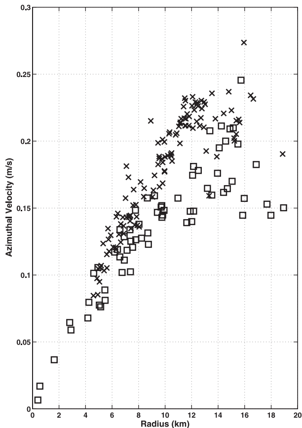
FIG. 8. Azimuthal velocities as a function of radius to SCV center for MV 19954 (crosses) and VCM RAFOs 30 (squares). One velocity estimate is provided by half rotation period around the center (center positions are estimated independently for the two floats).
