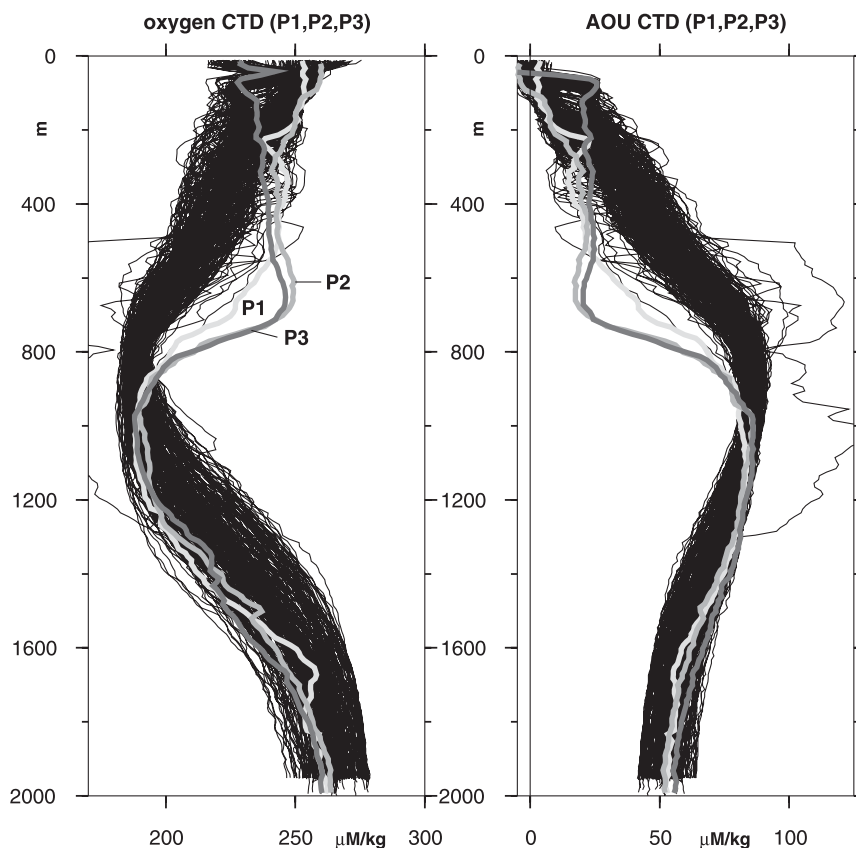
FIG. 5. Vertical profiles of dissolved oxygen ( \mu\text{M kg}^{-1} ) as a function of pressure from 0 to 2000 dbar for all CTD casts ( >80 ) taken during leg 1 of P1 (February), P2 (April), and P3 (September) in 2001. Also CTD casts 23 (leg1, P1), 41 (leg1, P2), 26 (leg 1, P3) collected in the SCV core (close to VCM 030 and MV 19954).
