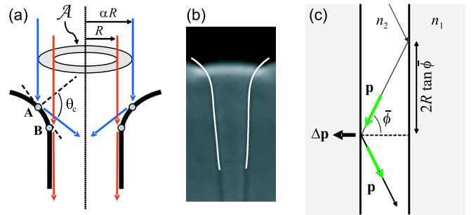
FIG. 4: (Color online) Illustration of the geometrical model of optical bridge stabilization (a) Rays impinging on the interface at an angle larger than \theta_c , the critical angle for total internal reflection, participate in stabilizing the bridge structure. (b) Picture of the funnel shape at the bridge entrance showing data analysis (white line) from which the parameter \alpha is estimated. (c) Linear momentum transfer \Delta\mathbf{p} of a photon that undergoes total internal reflection inside the bridge.
