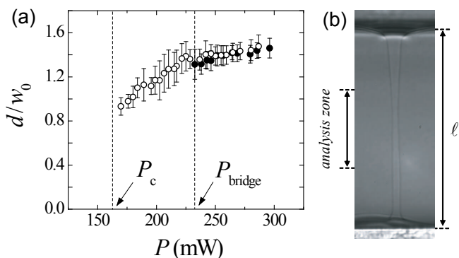
FIG. 3: (a) Bridge diameter as a function of power for w_0 = 6.95 \mu\text{m} for increasing (filled circles) and decreasing (open circles) power. P_c is the critical power below which the bridge is no longer stabilized by light. (b) Typical bridge obtained at 230 mW. The aspect ratio is \Lambda \approx 20 .
