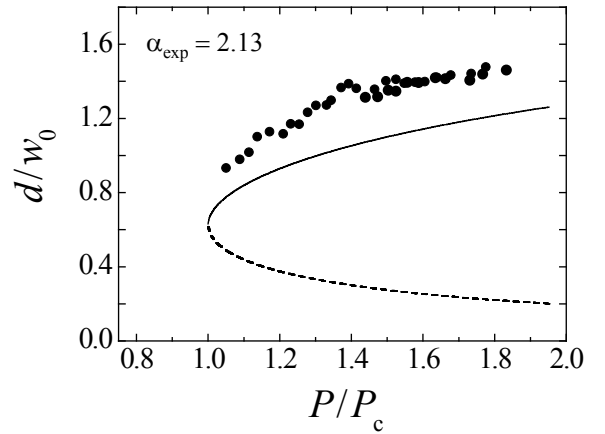
FIG. 6: Comparison between the model and experimental results for w_0 = 6.95 \mu\text{m} and T - T_c = 4 \text{ K} . Solid (dashed) line corresponds to stable (unstable) states and circles are the experimental results.
