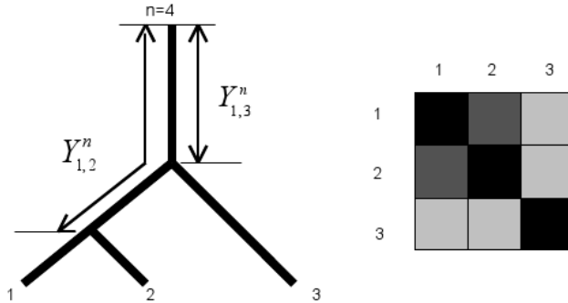
Figure 1. The distance Y_{i,j}^{n=4} between a reference taxa n and the path i - j on an X-tree fulfils Kalmanson inequalities. If the values of the distance matrix Y_{i,j}^{n=4} are coded in a gray scale, the level of gray decreases as one moves away from the diagonal. For more details see Thuillard (2007).
