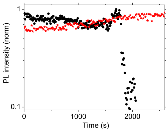
FIG. 1: Temporal evolution of the photoluminescence intensity (logarithmic scale) after deposition on a glass substrate of a suspension of SWCNTs in water (black dots) and a drop of gelatin-enriched material (red stars) at room temperature. The luminescence intensity of the gelatin-based sample remains constant over time whereas the luminescence of the suspension is reduced by one order of magnitude when the solvent is evaporated. The transient increase of the signal is likely due to a lens effect in the drying drop changing the collection efficiency of the setup.
