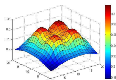
Figure 15. Current repartition with four contact zones. R_m = 3m\Omega
