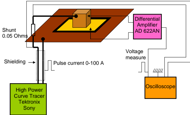
Figure 5. Current pulse generation and measuring chain
