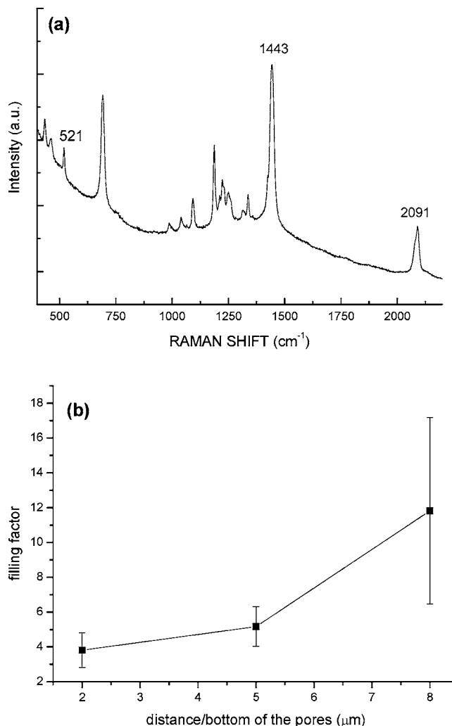
Figure 2. (a) Resonance Raman spectra of monomer inside the pores. (b) Concentration profile of the monomer inside the porous silicon layer obtained by Raman scattering spectroscopy on a cleaved layer. The filling factor corresponds to the peak area \delta_{\text{COH}}/\nu_{\text{Si}} ratio.
