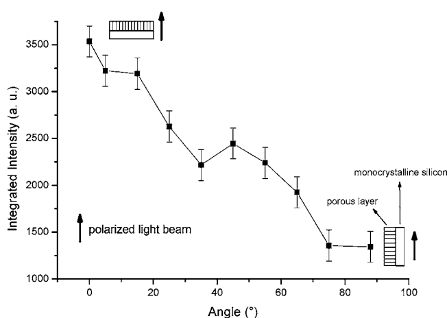
Figure 4. Intensity evolution of the 2091 \text{cm}^{-1} band as a function of monomer orientation inside a porous silicon layer measured by polarized Raman scattering spectroscopy ( \lambda = 676.4 \text{ nm} ).
