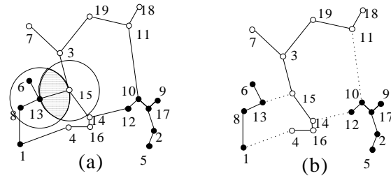
Figure 1: RNG and clusters with two classes: the black and the white points
