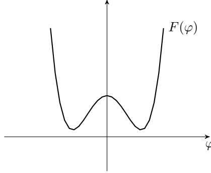
Figure 2: Possible shape of the potential F(\varphi)
