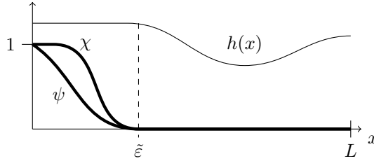
Figure 4: Possible shapes of function \chi and \psi
