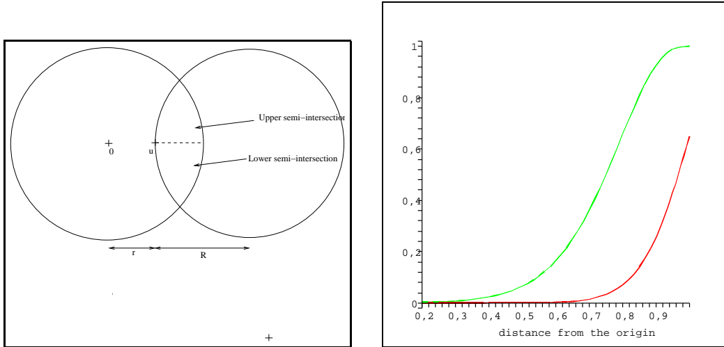
(a) The two semi-intersections used in the proof of Proposition 4. (b) Lower and upper bounds on the probability of belonging to MPR_1 w.r.t. the distance from 0.
