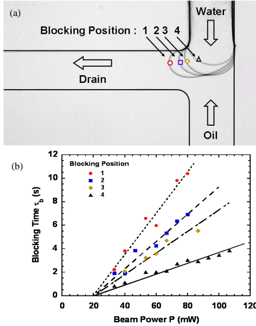
Figure 1: Microfluidic valve in a T geometry. (a) Superposition of microscopic images of the laser blocking the interface at different locations in the microchannel. All channels are 100\ \mu\text{m} wide. (b) Dependence of the blocking time \tau_b on laser power and position (indicated in (a)) for Q_{\text{oil}} = 0.05\ \mu\text{L}/\text{min} and P_{\text{water}} = 2.3 \times 10^3\ \text{Pa} , \omega_0 = 2.6\ \mu\text{m} . The lines are linear fits to guide the eye.
