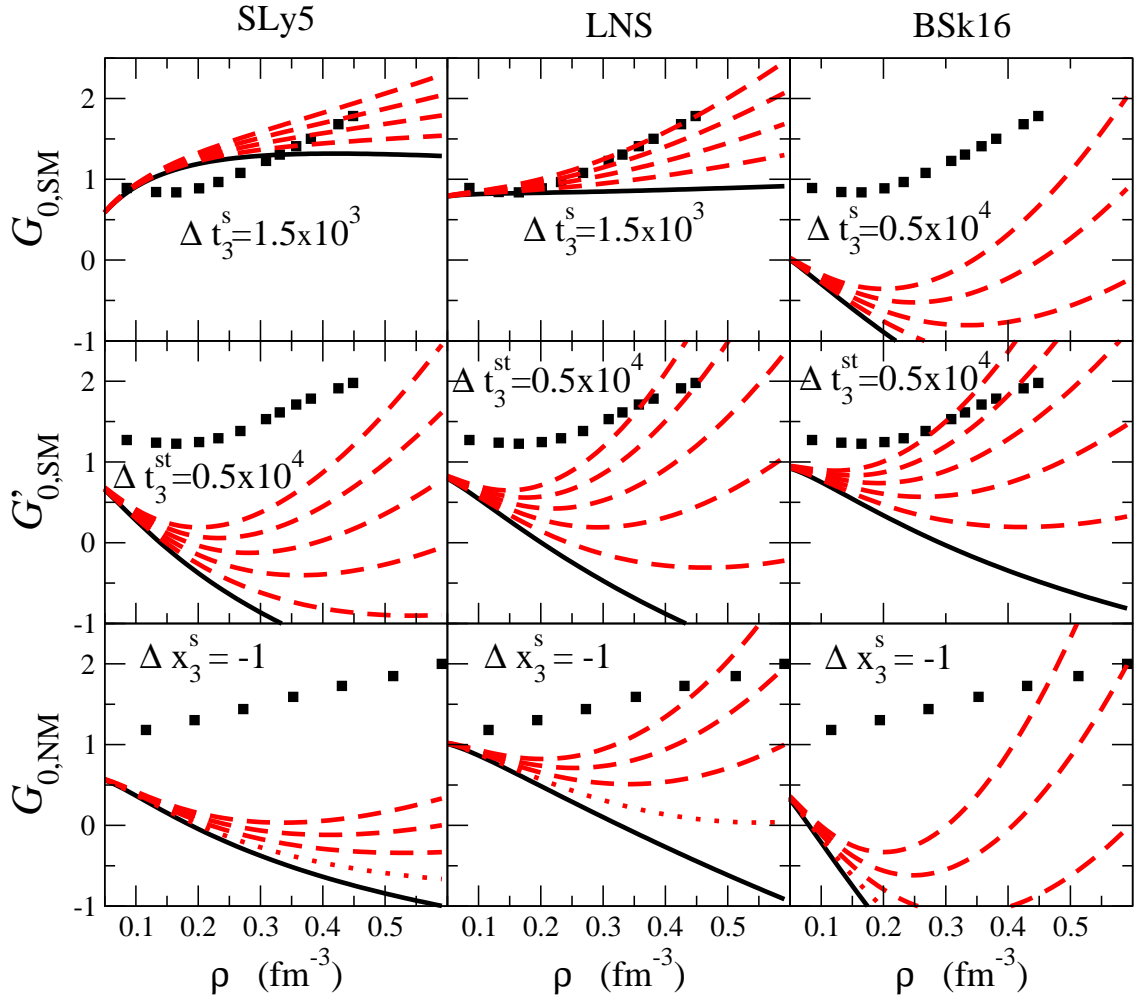
Figure 3. Landau parameters for spin and spin-isospin channels G_0 and G'_0 in symmetric nuclear matter and neutron matter. The solid curves are the original ones, while the filled squares are obtained by the Brueckner HF calculations as shown in Fig. 2. The dashed curves correspond to different values of the parameters t_3^s , t_3^{st} and x_3^s . The parameters are changed from bottom to top multiplying integers (1,2,3,-) by the mesh size given in each window. The Landau parameter G_{0,NM} is calculated with the optimal value for t_3^s in Tab. 2, which reproduces best the Brueckner HF G_{0,SM} values. The thin dotted lines in the bottom panels correspond to the results with x_3^s=0 .
