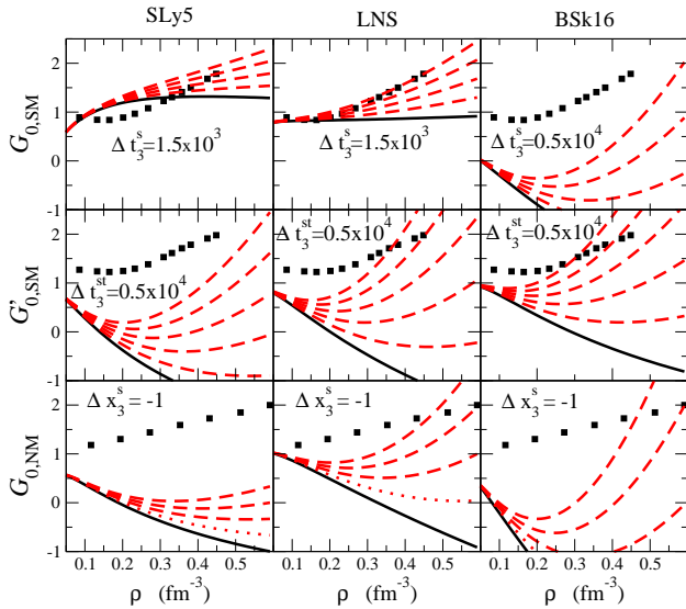
FIG. 3: (color online) Landau parameters for spin and spin-isospin channels G_0 and G'_0 in symmetric nuclear matter and neutron matter. The solid curves are the original ones, while the filled squares are obtained by the Brueckner HF calculations as shown in Fig. 2. The dashed curves correspond to different values of the parameters t_3^s , t_3^{st} and x_3^s . The parameters are changed from bottom to top multiplying integers (1,2,3,-) by the mesh size given in each window. The Landau parameter G_{0,NM} is calculated with the optimal value for t_3^s in Tab. I, which reproduces best the Brueckner HF G_{0,SM} values. The thin dotted lines in the bottom panels correspond to the results with x_3^s=0 .
