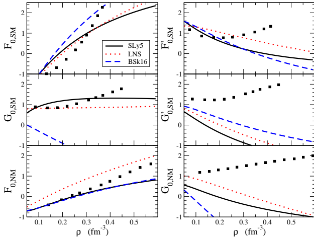
FIG. 2: (color online) Landau parameters in symmetric nuclear matter (SM) and neutron matter (NM) as a function of the density \rho obtained by the Skyrme interactions and the Brueckner HF calculations using 2BF+3BF [18]. Solid line for SLy5, dotted line for LNS, dashed line for BSk16 and filled squares for Brueckner HF calculations.
