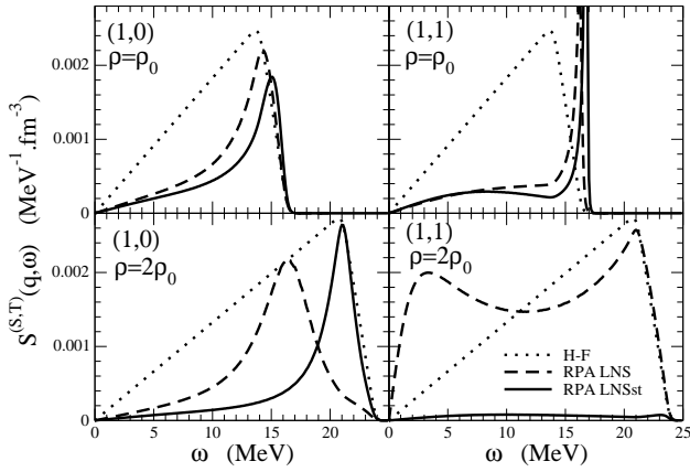
FIG. 4: RPA response functions S^{(S,T)}(q, \omega) for q=0.22 \text{ fm}^{-1} with the temperature T=0 \text{ MeV} calculated with LNS and LNSst interactions. Top panels are calculated for (S, T) = (1, 0) and (1, 1) with \rho = \rho_0 and bottom panels are for the same channels with \rho = 2\rho_0 .
