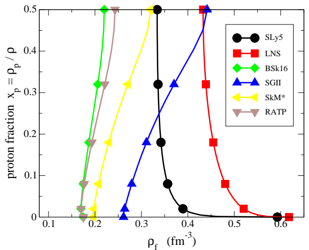
FIG. 1: (color online) Ferromagnetic phase diagram for various effective Skyrme interactions. The horizontal axis shows the critical density \rho_f at which the asymmetric matter becomes unstable, while the vertical axis shows the proton fraction x_p = \rho_p/\rho . The matter is spin symmetric for smaller density than \rho_f , while it becomes ferromagnetic for larger density than \rho_f . See the text for details.
