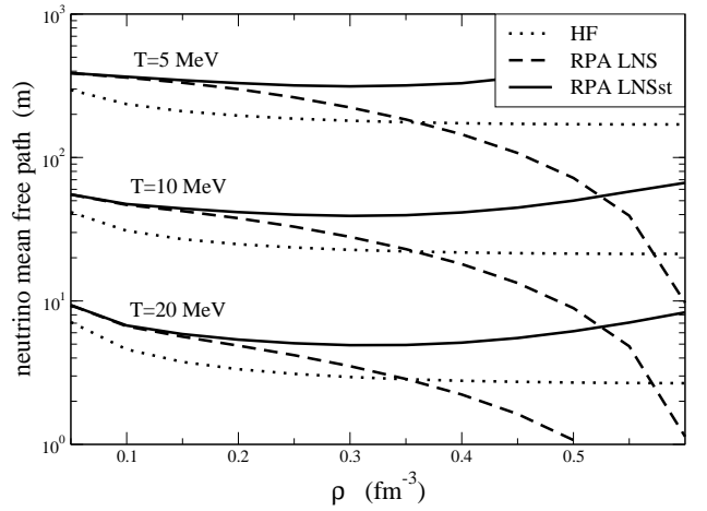
FIG. 5: Neutrino mean free path in neutron matter for different temperatures T=1, 10 and 20 \text{ MeV} . The neutrino energy is set to be E_\nu = 3T . The mean free path is calculated with the LNS Skyrme interaction by the HF mean field approximation (dotted line), including the RPA correlations with the original LNS interaction (dashed line) and RPA with the modified spin channel in LNSst (thick line).
