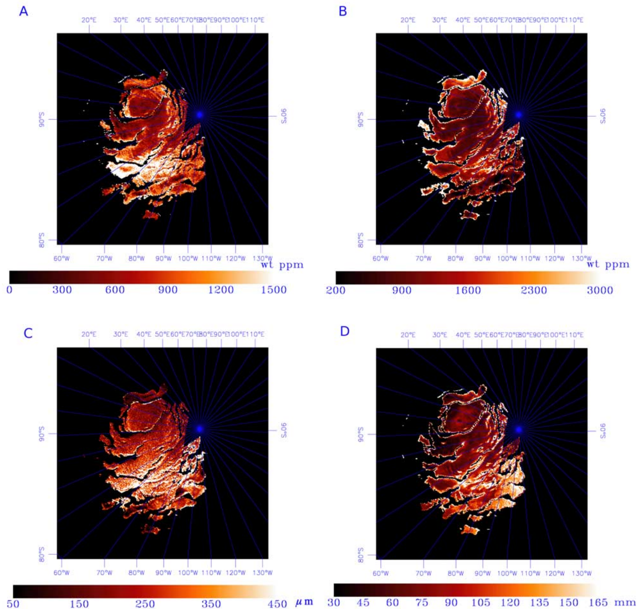
Figure 10. Global mosaics illustrating the absolute variations of (a) water ice and (b) dust proportions, as well as (c) water ice and (d) \text{CO}_2 ice grain sizes across the entire permanent bright polar cap. They are derived from individual parameter maps obtained by inverting OMEGA observations 41, 61, and 103 with GRSIR.
