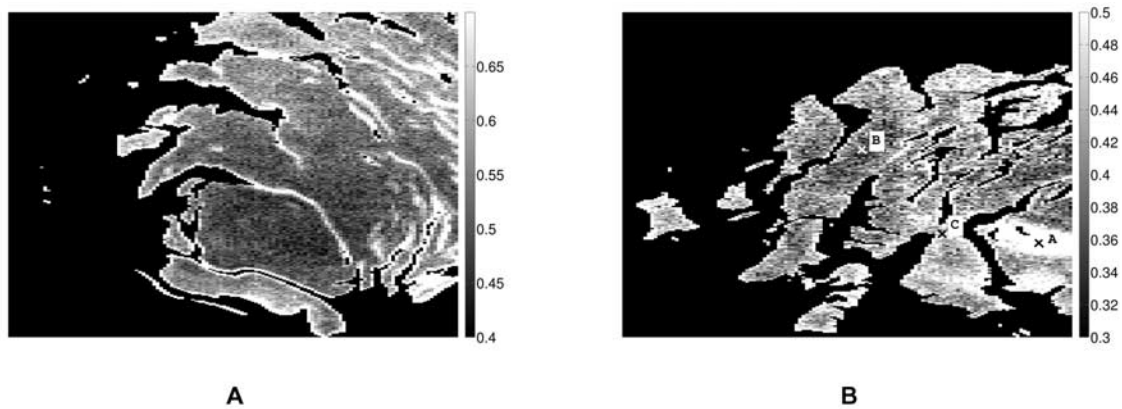
Figure 8. Cosines of the wavellet angle between the observed spectra and a reference spectrum of Martian dust for the hyperspectral images acquired during (a) orbit 41 and (b) orbit 103.
