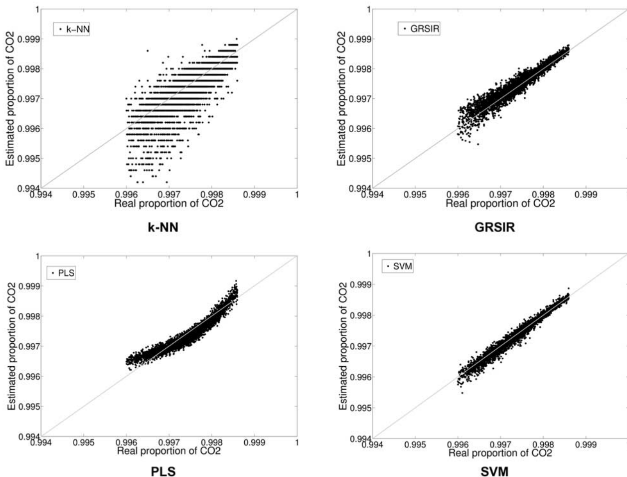
Figure 5. Scatterplots of estimated proportions of CO 2 ice by k -NN, GRSIR, PLS, and SVM (vertical axis) versus the proportion of CO 2 ice from the test data (horizontal axis).
