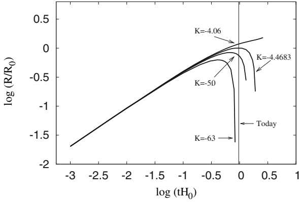
Fig. 1. Evolution of shells with different energies K .
