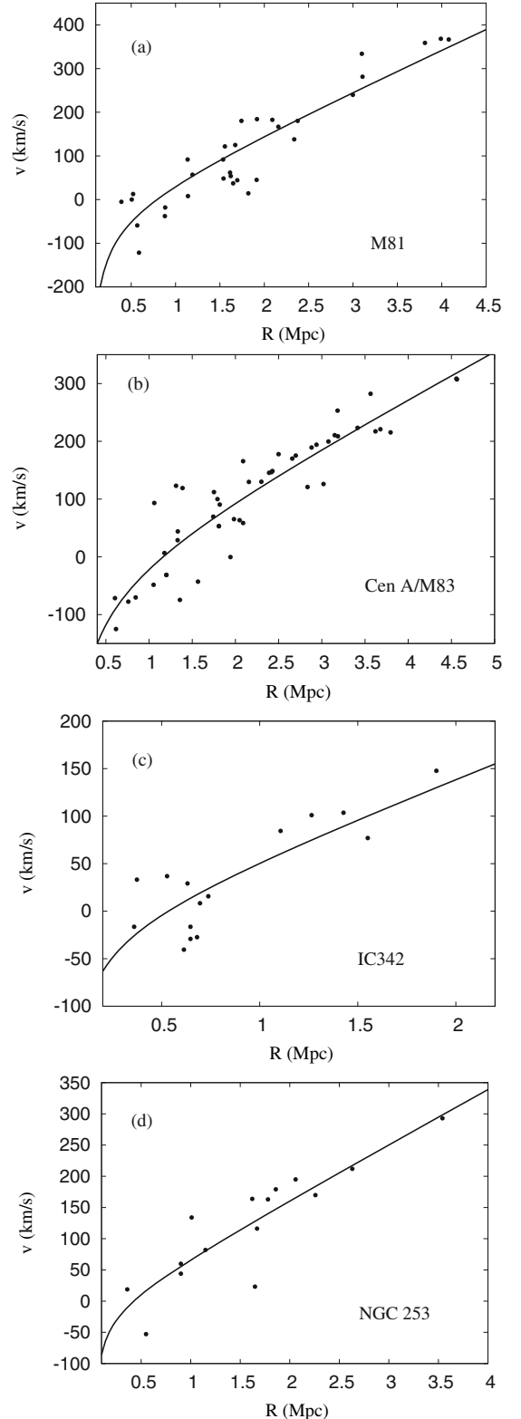
Fig. 2. Velocity-distance diagrams based on available data relative to a) the M81 group, b) the CenA/M83 complex, c) the IC342/Maffei-I group and d) the NGC 253 group. Solid lines are best fit to Eq. (7).
