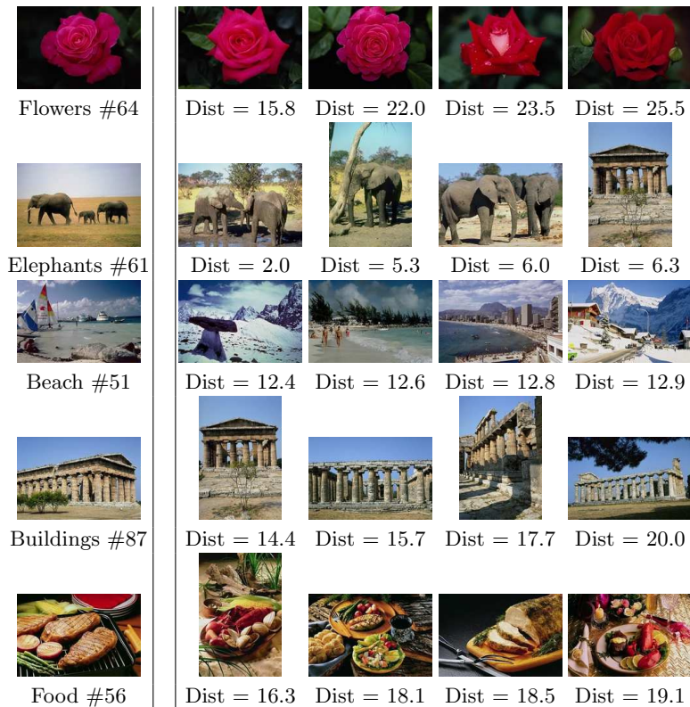
Fig. 7. Retrieval results for 5 images of the COREL database. For each row, left to right: query image; first 4 ranked images of the database (excluding the query image). For each retrieved image, the SMP similarity measure to the query is also shown.
