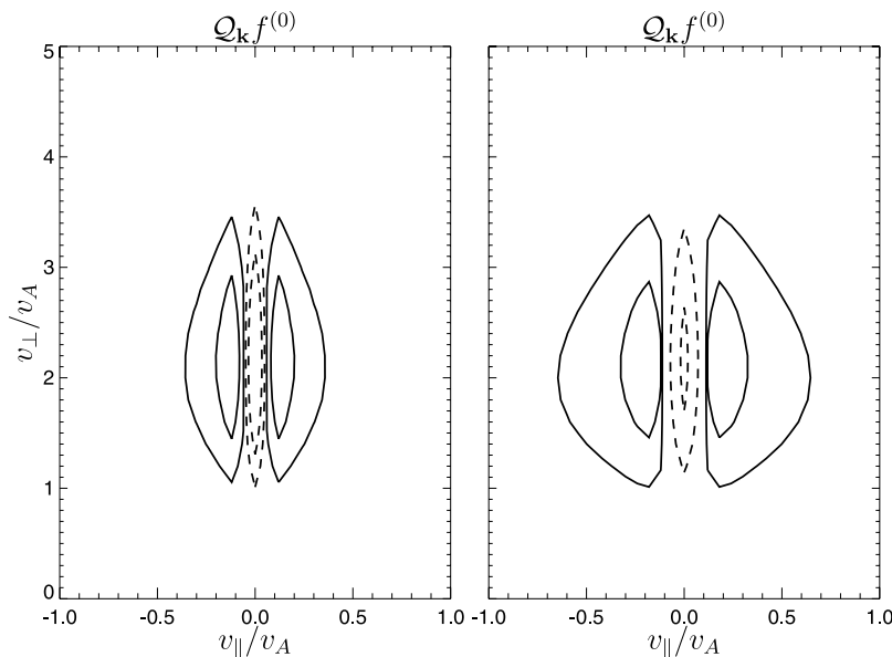
Figure 5. Schematic view of the prediction of the quasi-linear theory: Effect of the diffusion operator on the initial proton distribution function Q_{\mathbf{k}}f^{(0)} (left) for the most unstable mode and (right) for a weakly unstable mode. Solid (dashed) contours show positive (negative) values.
