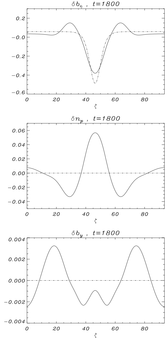
Figure 13. Persistence of initial perturbations in the form of a (top) magnetic hole and (middle) resulting density hump for \beta_{\parallel} = 6 and T_{\perp}/T_{\parallel} = 1.36 , with \theta = 83.82^\circ . The bottom panel displays the magnetic field component in the direction perpendicular to the plane defined by the ambient field and the direction of spatial variation.
