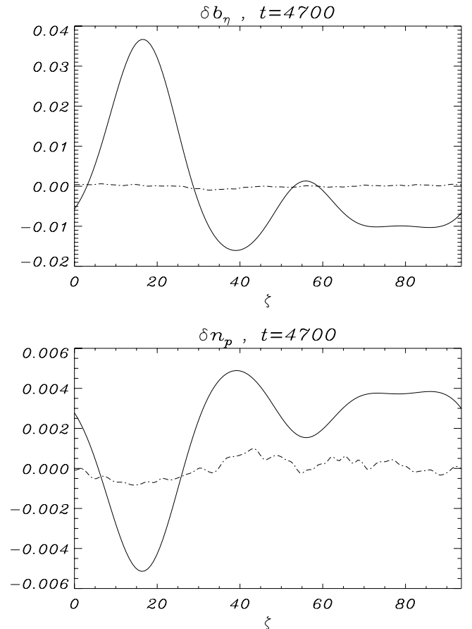
Figure 7. Magnetic humps and density holes formed as the development of the mirror instability presented in Figure 6. Here and in the following figures displaying results of the Eulerian simulations, dashed lines refer to initial conditions and solid lines to the final time of the simulations.
