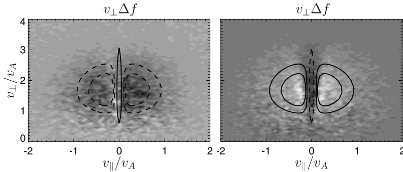
Figure 3. Same conditions as Figure 1. Gray scale plots of v_{\perp} \Delta f averaged over regions where (left) \delta B_{\eta}/B_0 > 0.01 and (right) \delta B_{\eta}/B_0 < -0.01 , at time t = 1000/\Omega_p . White corresponds to positive values and black to negative ones. Superimposed are the contours of the linear prediction, v_{\perp} f^{(1)} , at maximum (left) and, symmetrically, minimum (right) of B_z^{(1)} , for the most unstable mode. Solid and dashed lines denote positive and negative values of v_{\perp} f^{(1)} , respectively.
