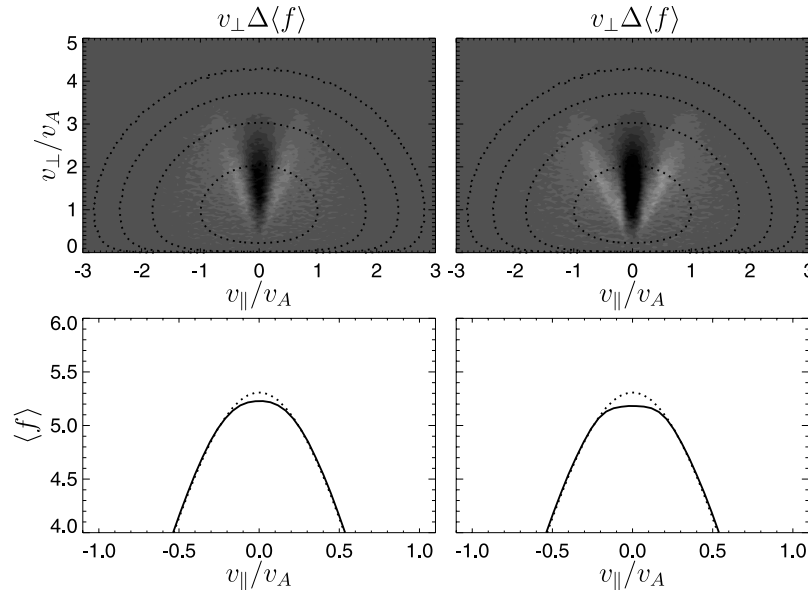
Figure 4. Same conditions as Figure 1. Simulation results at times (left) t = 2000/\Omega_p and (right) t = 10,000/\Omega_p : (top) Gray scale plots of the proton distribution variation v_{\perp}\Delta\langle f \rangle (black corresponds to negative values and white to positive ones). Dotted lines correspond to the contours of the initial condition v_{\perp}f^{(0)} . (bottom) Profiles (solid line) of the proton distribution function \langle f \rangle integrated over v_{\perp} , together with the initial profile (dotted line).
