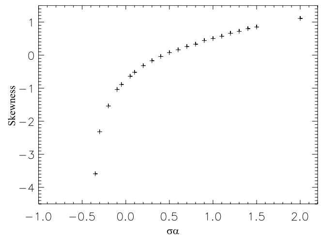
Figure 11. Variation of the skewness with the parameter \sigma\alpha , as predicted by the phenomenological model.
