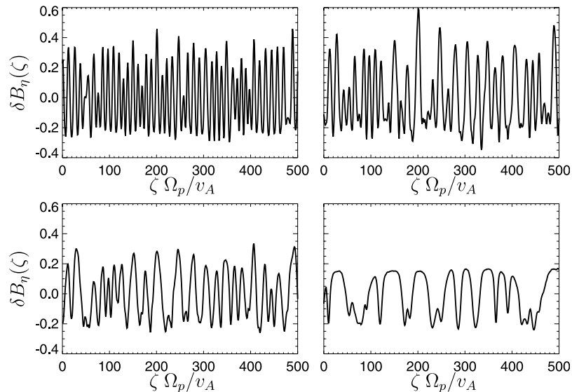
Figure 17. Profiles of \delta B_{\eta} as a function of \zeta in a fraction of the simulation box, in the conditions of Figure 16. From left to right and top to bottom: t = 60/\Omega_p , t = 100/\Omega_p , t = 150/\Omega_p , and t = 600/\Omega_p .
