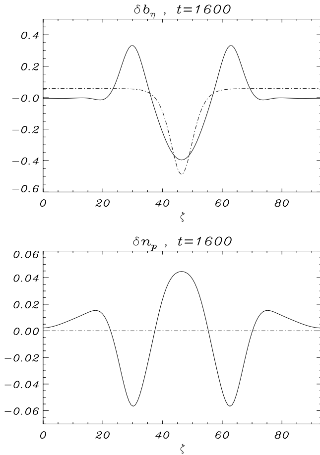
Figure 14. Persistence of a (top) magnetic hole and (bottom) resulting density hump at relatively large distance from threshold ( \beta_{\parallel} = 15 , T_{\perp}/T_{\parallel} = 1.5 , with \theta = 83.82^{\circ} ).
