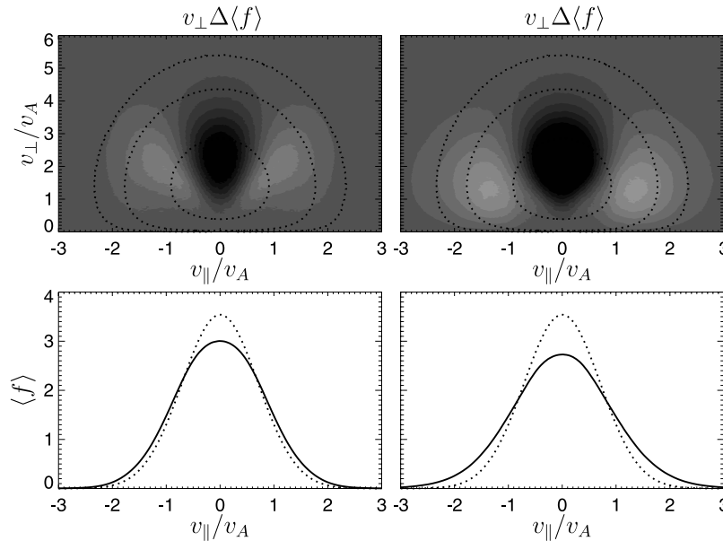
Figure 18. Same conditions as Figure 16. Simulation results at times (left) t = 60/\Omega_p and (right) t = 100/\Omega_p : (top) Gray scale plots of the proton distribution variation v_{\perp}\Delta\langle f\rangle (black corresponds to negative values and white to positive ones). Dotted lines correspond to the contours of the initial condition v_{\perp}f^{(0)} . (bottom) Profiles (solid line) of the proton distribution function \langle f\rangle integrated over v_{\perp} , together with the initial profile (dotted line).
