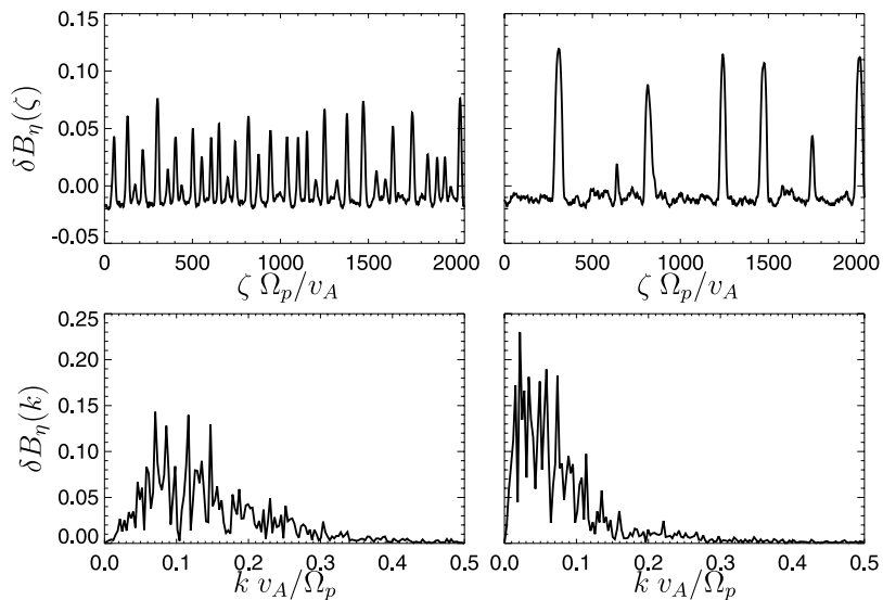
Figure 2. Same conditions as Figure 1. (top) Profile and (bottom) spectrum of \delta B_{\eta} at times t = 2000/\Omega_p (left) and t = 10000/\Omega_p (right).
