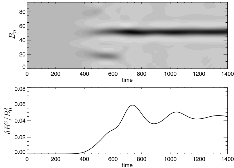
Figure 9. Grey scale plot of the magnetic fluctuations B_\eta as a function of space and time and time evolution of the magnetic-energy fluctuations \delta B^2/B_0^2 in the conditions of Figure 8.
