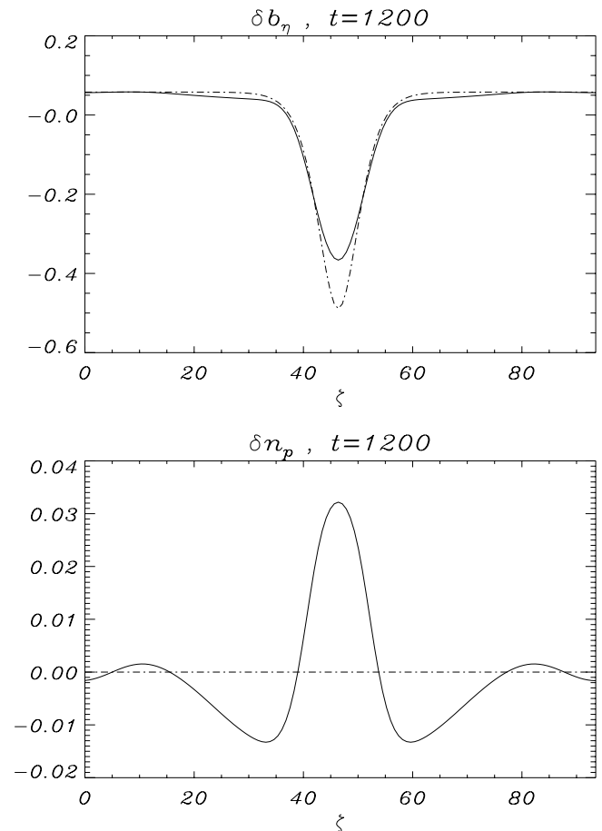
Figure 15. Persistence of a (top) magnetic hole and (bottom) resulting density hump, in a plasma with T_{\perp} = T_{\parallel} and \beta_{\parallel} = 6 , with \theta = 83.82^{\circ} .
