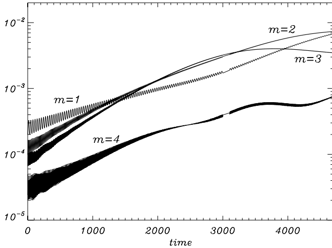
Figure 6. Time evolution of unstable modes in an Eulerian simulation very near threshold ( \beta_{\parallel} = 6 , temperature anisotropy T_{\perp}/T_{\parallel} = 1.25 , with \theta = 83.86^{\circ} ).
