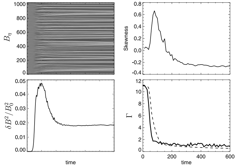
Figure 16. Evolution in an extended domain, for \beta_{\parallel} = 1 , T_{\perp}/T_{\parallel} = 4 and \theta = 50.5^{\circ} . Gray scale plot of the magnetic fluctuation B_{\eta} as a function of time and space (left top); Time evolution of skewness of B_{\eta} (right top), of fluctuating magnetic energy \delta B^2/B_0^2 (left bottom), of the instantaneous distance from the threshold (right bottom): \Gamma (solid line) as given by equation (1) and the corresponding bi-Maxwellian value \Gamma^* (dashed line) obtained from equation (2).
