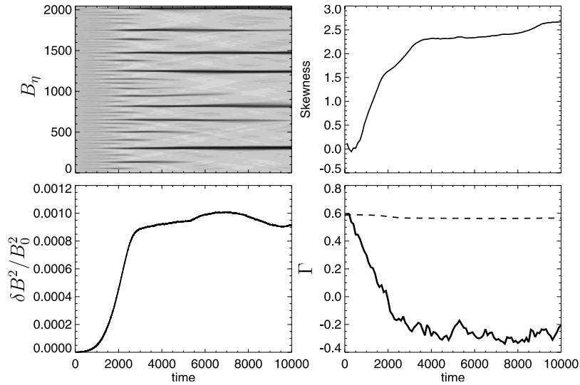
Figure 1. Simulation of the mirror instability in an extended domain near threshold ( \beta_{\parallel} = 1 , T_{\perp}/T_{\parallel} = 1.857 , and \theta = 72.8^{\circ} ). Gray scale plot of the magnetic fluctuation B_{\eta} as a function of time and space (left top); Time evolution of skewness of B_{\eta} (right top), of fluctuating magnetic energy \delta B^2/B_0^2 (left bottom), of the instantaneous distance from the threshold (right bottom): \Gamma (solid line) as given by equation (1) and the corresponding bi-Maxwellian value \Gamma^* (dashed line) obtained from equation (2).
