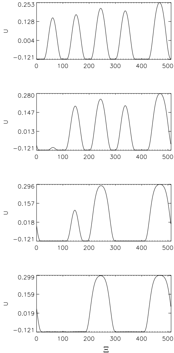
Figure 10. Time evolution of magnetic structures resulting from the mirror instability in the framework of the phenomenological model for \alpha = 1.54 , \nu = 10^{-2} and a weak initial noise. Panels are displayed at times t = 3, 5, 9 , and 10 (from top to bottom). The horizontal axis refers to grid point numbers.
