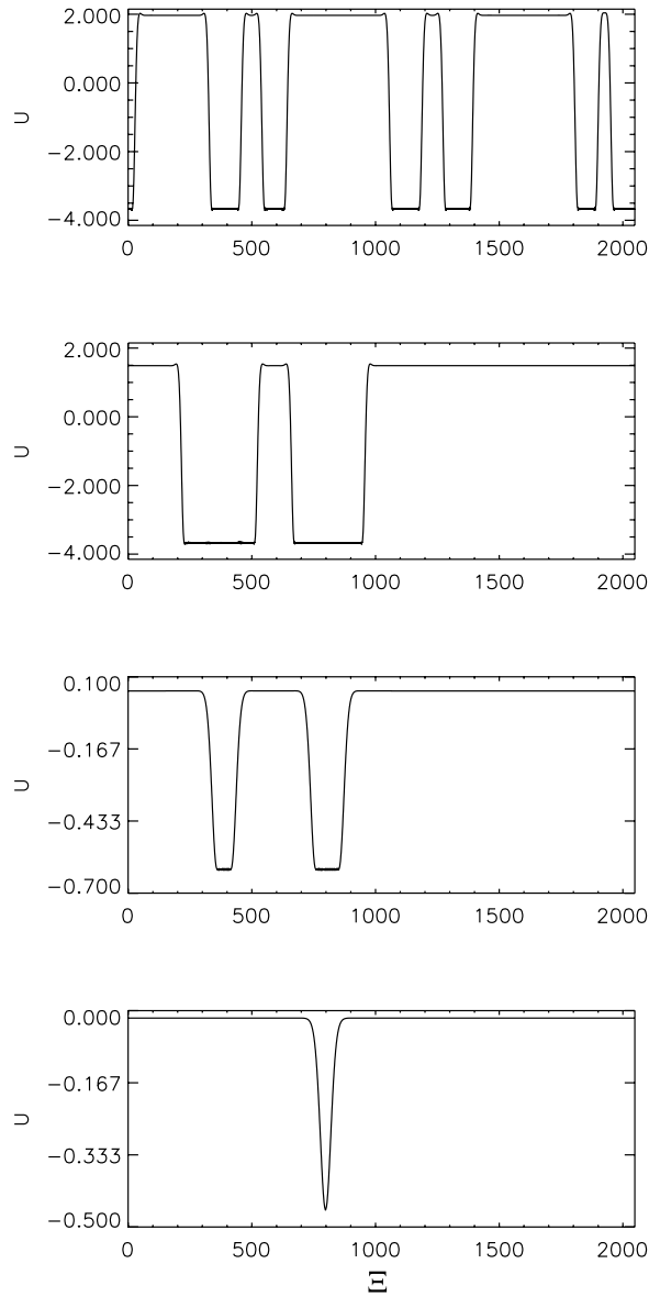
Figure 12. Magnetic holes predicted by the phenomenological model for \sigma\alpha = 0.05, -0.05, -0.3, -0.4 (from top to bottom), when initialized with a random noise of small amplitude when \sigma = +1 (over threshold) and of large amplitude when \sigma = -1 (below threshold).
