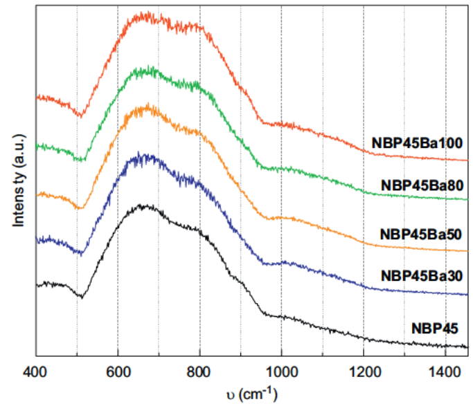
Fig. 2. Raman spectra for glasses NBP45, NBP45Ba30–Ba100.
