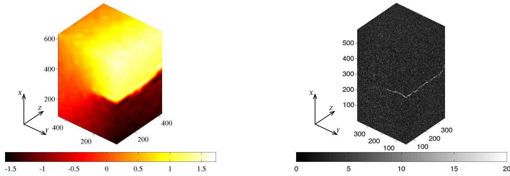
Figure 19. Displacement component (expressed in voxels) along the loading direction obtained from Digital Image Correlation using C8 elements whose size is \ell = 32 voxels (left). Corresponding residual field (right). Its level should be compared to the dynamic range of the pictures ( i.e. , 256 gray levels). The voxel size is 3.5 \mu\text{m} .
