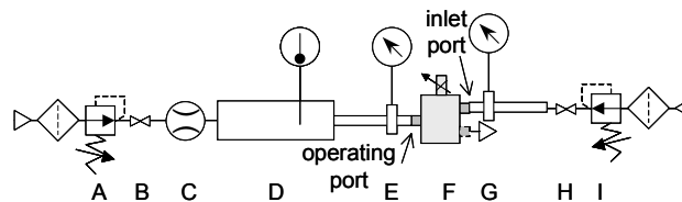
b) Exhaust flow rate-pressure characterisation
