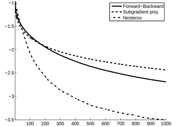
Fig. 2. Decay with k of the error \log_{10}(\|f^{(k)} - f^*\|/\|f^*\|) for the one-step forward-backward dual projection in Algorithm 1 (solid line), for the multi-step dual projection in Algorithm 2 (dashed-dotted line), and the sub-gradient projection [12] (dashed line). Here \tau = \|f_0\|_{\text{TV}}/4 .
