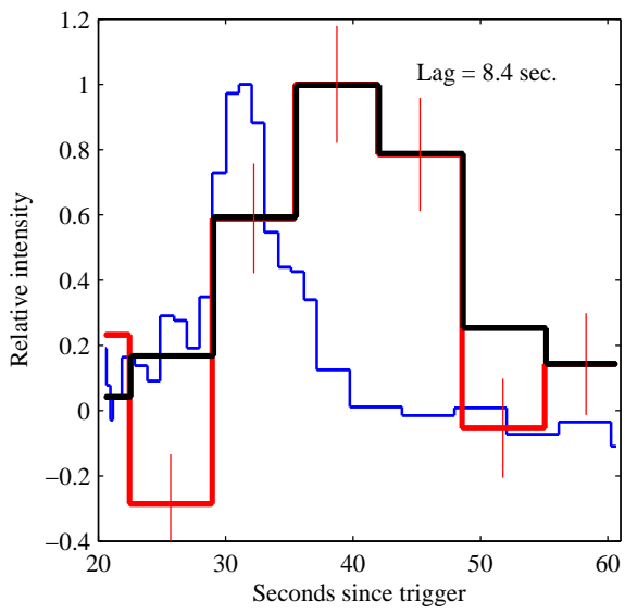
Fig. 4.— The convolution of the peak of BAT light curve (in blue) by the PSF-TAROT shifted by 8.4s (in black) compared to the TAROT data (in red). This figure appears in colors in the electronic version.
