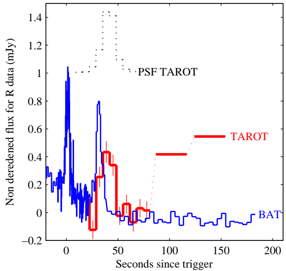
Fig. 3.— Light curves of GRB 081126 measured by BAT and TAROT. The dotted line labeled 'PSF-TAROT' stands for the spread of a star equivalent to an instantaneous flash of 0s duration. This figure appears in colors in the electronic version.
