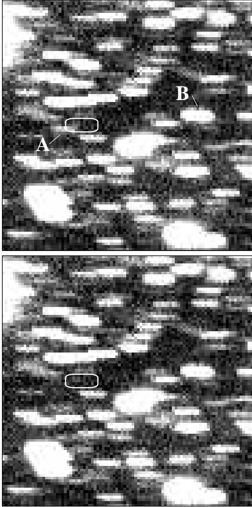
Fig. 1.— Field of GRB 081126. Top: TAROT image taken between 21s and 81s after the GRB trigger. The hour angle velocity was adapted to obtain stars as trails of \sim 9.2 pixel length during the 60s exposure. The theoretical position of the GRB trail is indicated by the white box. The star A covers partly the GRB trail. (see text). Bottom: After subtraction of star A using the model of star B, the trace of the optical emission of the GRB appears in the box. The image size is 5 arcmin, North is up, East left.
