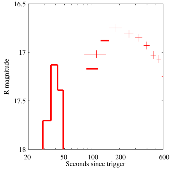
Fig. 2.— Optical light curve of GRB 081126. TAROT optical data are thick bars and observations from Skvarc & Mikuz (2008) are thin bars (2 sigma level). There are data in the ranges 20–29 and 49–89 sec, but with no detection at the limit of R=18.0 .
