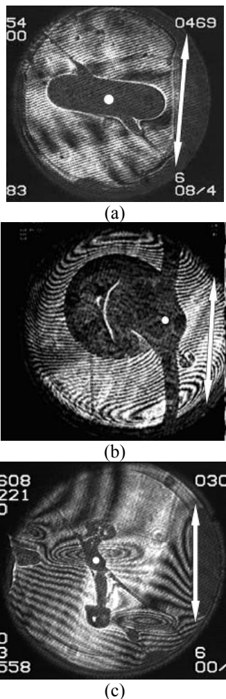
Fig. 1 The structure of heat and mass transfer from a point heater (ALICE-1,2 space experiments). (a) thermovibrational regime, (b) combined regime, and (c) thermoinertial regime. White arrows denote the direction of maximum variation of the microacceleration vector, and white circles denote the location of the heater.
