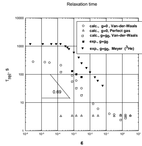
Fig. 8 Relaxation time as a function of the proximity to the critical point \varepsilon = (T-T_c)/T_c .
