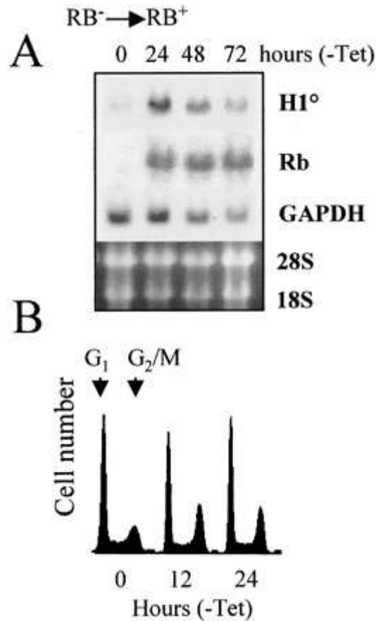
FIG. 7. RB modulates the expression of the endogenous H1 o gene. The RB-deficient SAOS-2 cell line, harboring an inducible RB-encoding transgene, was cultured in the absence of tetracycline to induce the expression of RB. (A) At the indicated times, RNA was prepared from these cells, and the Northern blot obtained was probed successively with 32 P-labeled H1 o , RB, and GAPDH probes. The ethidium bromide-stained gel before the transfer of RNAs onto the membrane is shown. (B) The induced accumulation of RB is associated with the modification of cell cycle parameters. SAOS-2 cells were fixed at the indicated times after the removal of tetracycline, stained with propidium iodide, and analyzed using a flow cytofluorimeter. Histograms represent the number of cells as a function of DNA content (DNA fluorescence).
