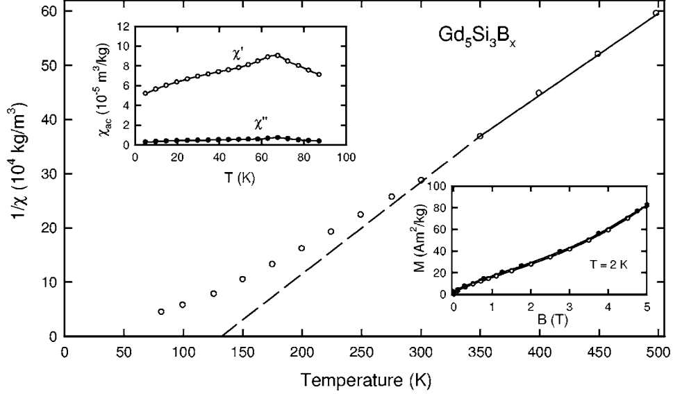
Fig. 3. Reciprocal susceptibility versus temperature for \text{Gd}_5\text{Si}_3\text{B}_x . Upper inset: ac and dc susceptibilities versus temperature. Lower inset: isothermal magnetization versus external field (open circles field up, filled symbols field down).
