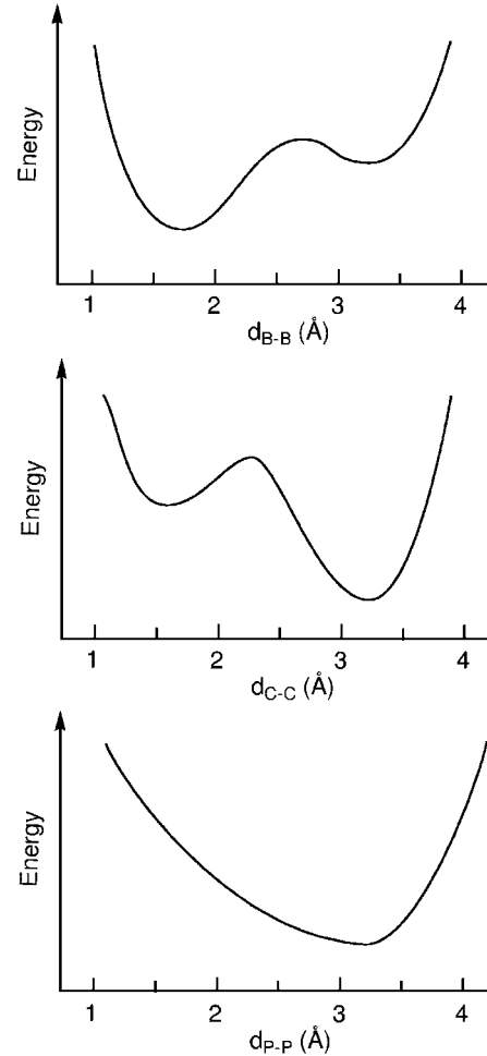
Fig. 19. Schematic potential energy curves as a function of Z–Z distance in Gd_5Si_3Z : Z = B (top), C (middle) and P (bottom).
