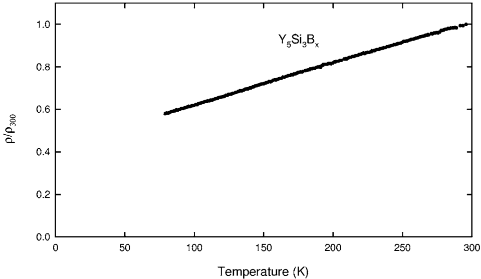
Fig. 17. Electrical resistivity vs temperature for Y_5Si_3B_x .
