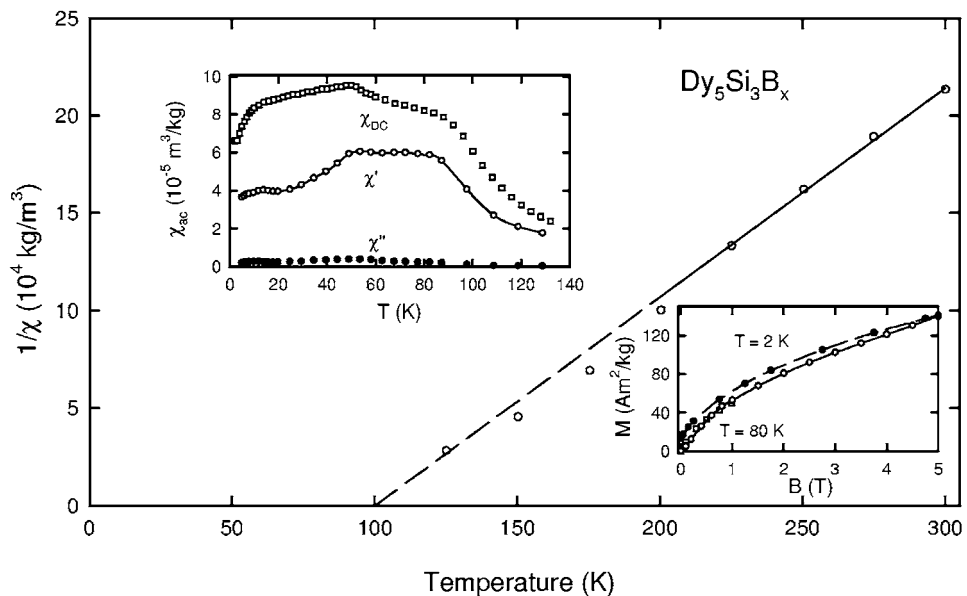
Fig. 11. Reciprocal susceptibility versus temperature for Dy 5 Si 3 B x . Upper inset: ac and dc susceptibilities versus temperature. Lower inset: isothermal magnetization versus external field (open symbols field up, filled symbols field down).
