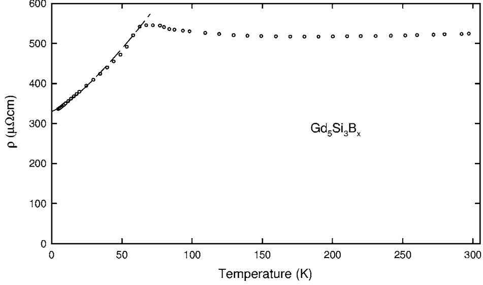
Fig. 5. Electrical resistivity versus temperature for \text{Gd}_5\text{Si}_3\text{B}_x . Dashed line calculated after Eq. (2).
