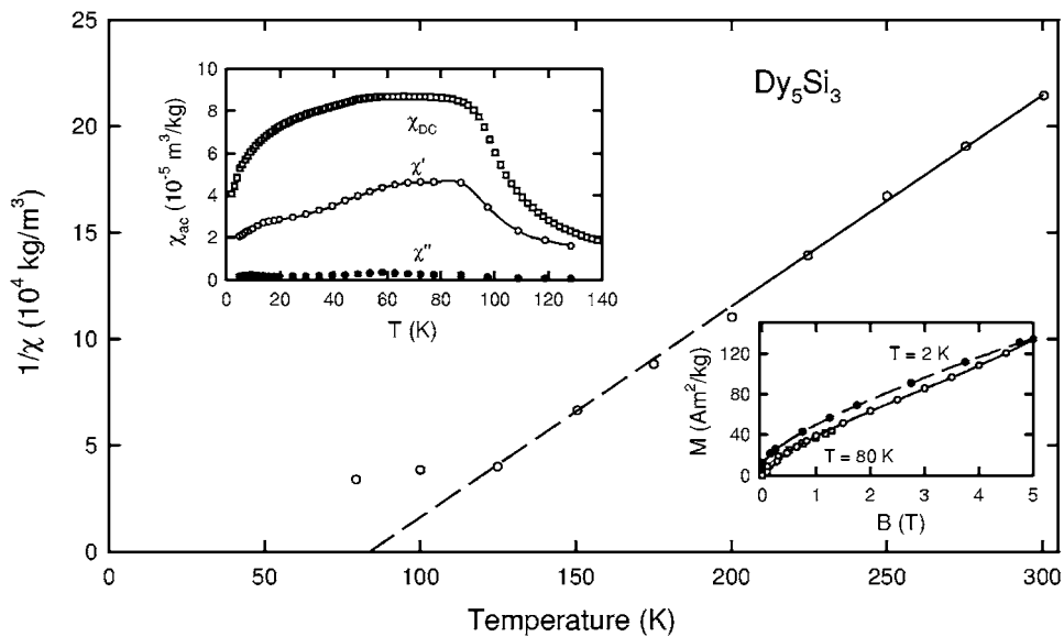
Fig. 10. Reciprocal susceptibility versus temperature for Dy 5 Si 3 . Upper inset: ac and dc susceptibilities versus temperature. Lower inset: isothermal magnetization versus external field (open symbols field up, filled symbols field down).
