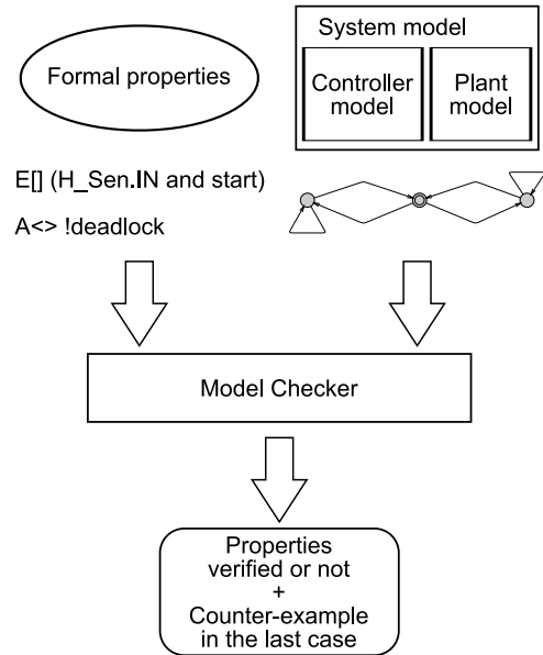
Fig. 1. Model-based model-checking principle
