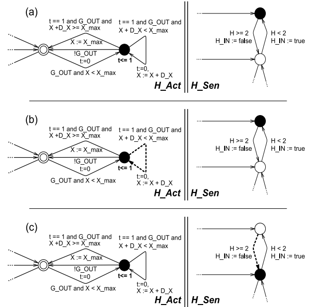
Fig. 6. Possible evolutions of H\_Act and H\_Sen , where the active locations are blocked.
