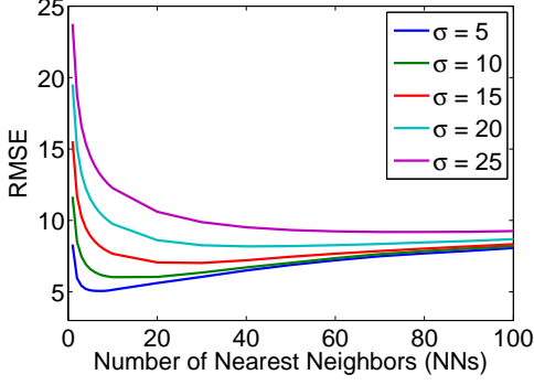
Fig. 1. RMSE in function of the numbers of nearest neighbors for different levels of noise.
