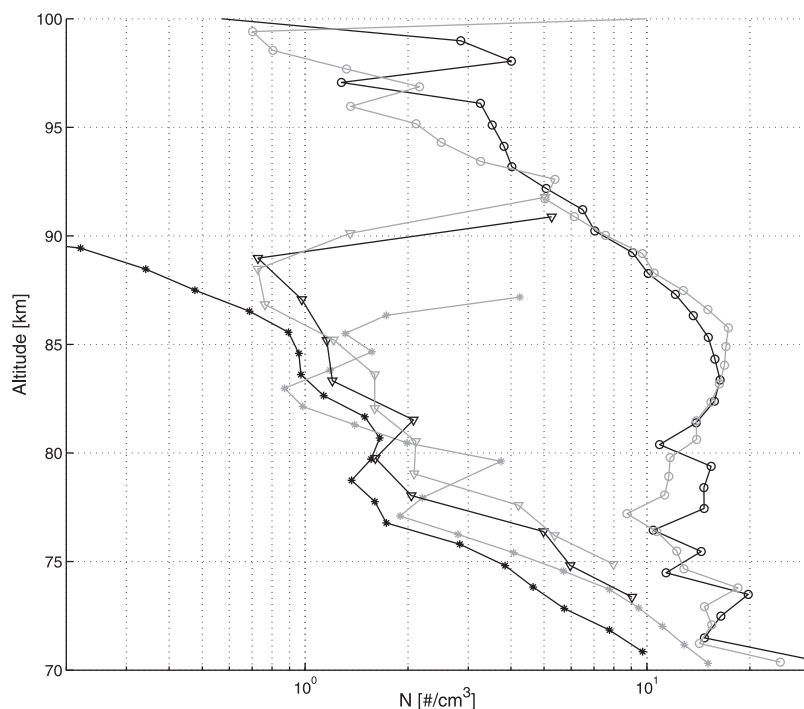
Figure 9. Vertical profiles of the particle total number density in the Venus upper haze during two successive orbits of Venus Express. The radius of particles found by fitting normalized extinction to a haze model allowed derive N for mode 1 particles with the SPICAV-UV channel (circles), N for mode 2 particles with the SPICAV-IR channel (inverted triangles), and N for mode 2 particles with the SOIR channel (asterisks) during orbit 485 (black) and orbit 486 (gray).
