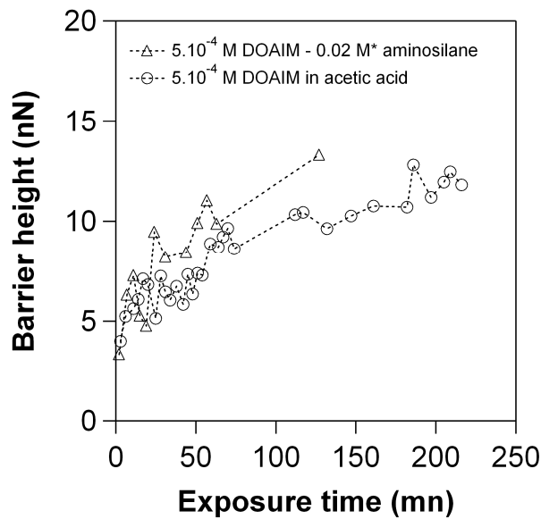
Figure 5. Surfactant compression forces evolution with exposure time of silica to (Δ) 5.10^{-4} M DOAIM – 0.02 M* aminosilane mixture (silane hydrolysis in pure water) and to (o) 5.10^{-4} M DOAIM in acetic acid.
