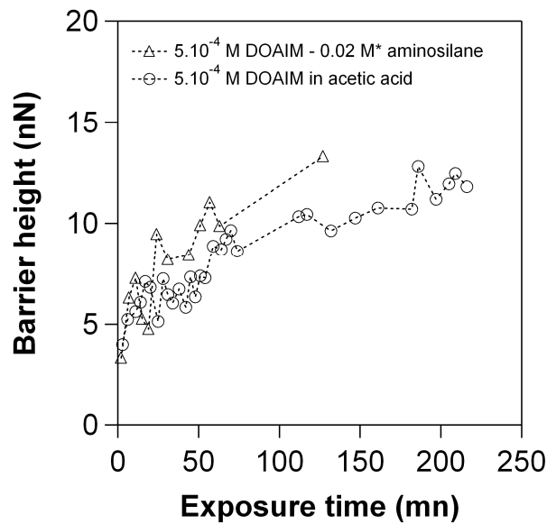
Figure 5. Surfactant compression forces evolution with exposure time of silica to (Δ) 5.10^{-4} M DOAIM – 0.02 M* aminosilane mixture (silane hydrolysis in pure water) and to (○) 5.10^{-4} M DOAIM in acetic acid.
