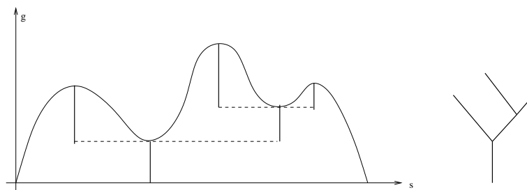
FIGURE 1. A height process g and its associated real tree
