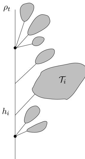
FIGURE 2. The measure \rho_t and the family (h_i, \mathcal{T}_i)_{i \in \mathcal{I}}
