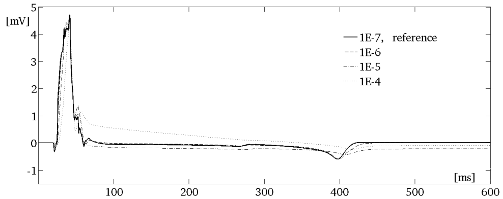
FIGURE 14. ECG recorded at electrode V1 using the bidomain model for various tolerances during the linear system inversion. ECGs depicted here correspond to a tolerance varying from 10^{-4} up to 10^{-7} . This last 10^{-7} tolerance corresponding to the reference solution of the bidomain model.
