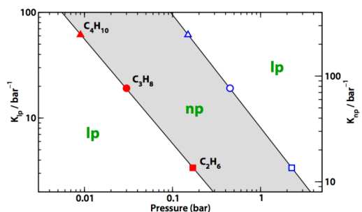
Figure 2: Existence domains of the lp and np phases of MIL-53 upon gas adsorption, with guests of different affinities ( K_{\mathbf{lp}} and K_{\mathbf{np}} ). Symbols correspond to lp → np and np → lp (respectively filled and open) transitions for the C 2 to C 4 alkanes.
