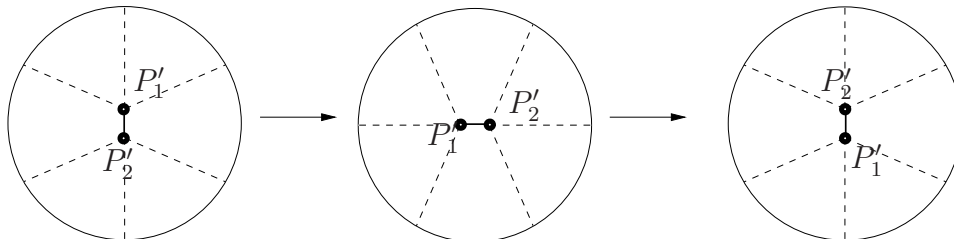
FIGURE 8. Interchanging two zeros of the same degree.
