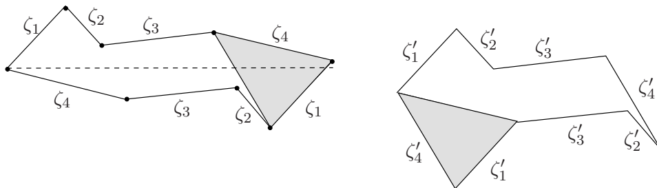
FIGURE 6. Rauzy-Veech induction on a suspension over an interval exchange transformation.
