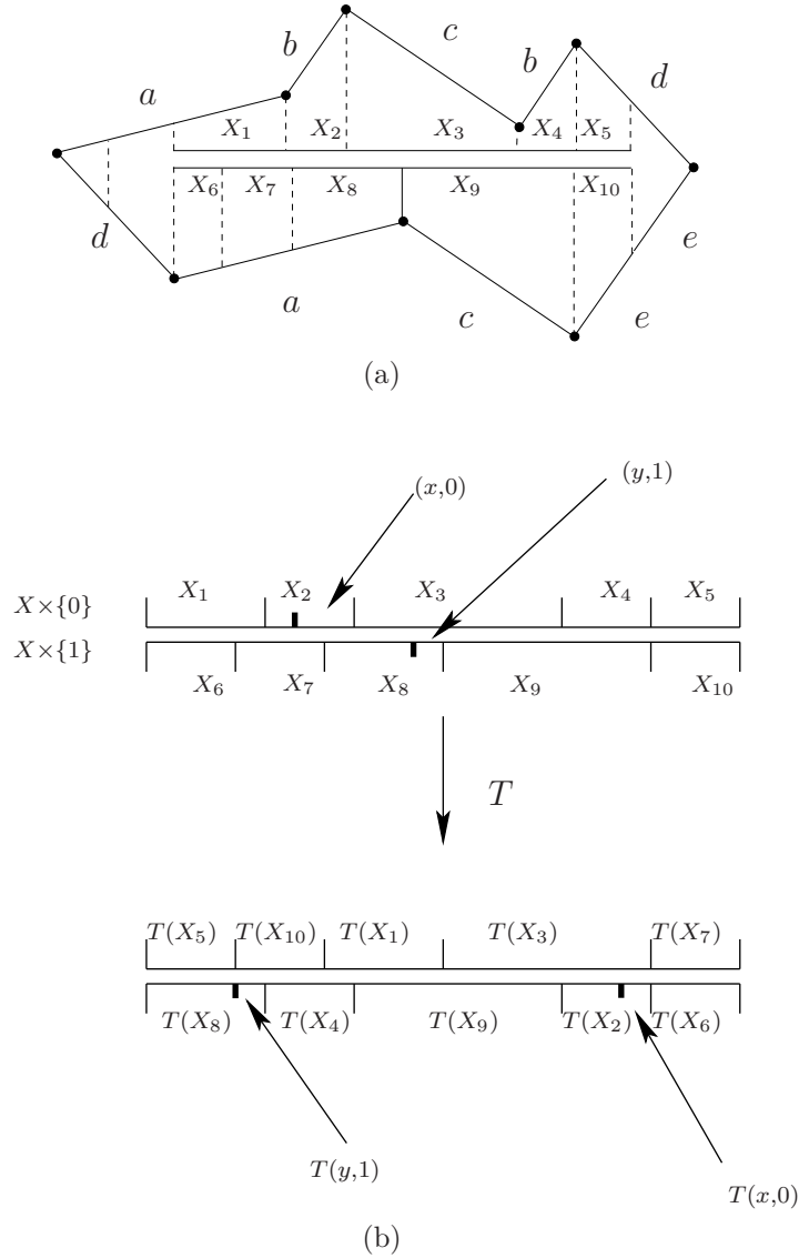
FIGURE 2. A linear involution associated to a measured foliation on a flat surface.
