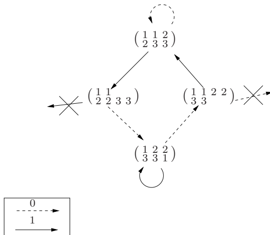
FIGURE 4. An example of a Rauzy diagram for generalized permutations.
