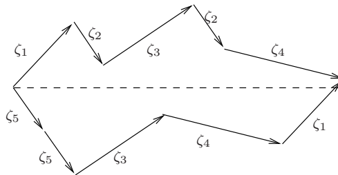
FIGURE 5. A suspension over a linear involution.
