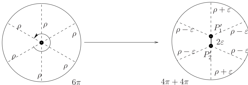
FIGURE 7. Breaking up a zero, after Eskin, Masur and Zorich
