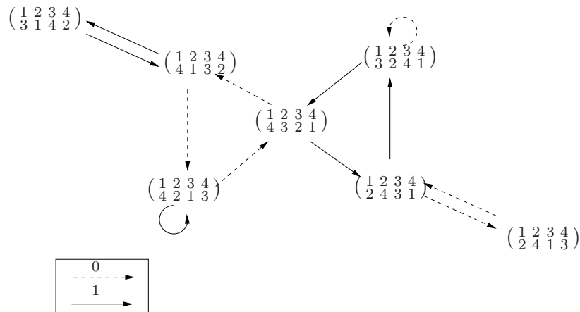
FIGURE 3. An example of a Rauzy diagram for permutations.
