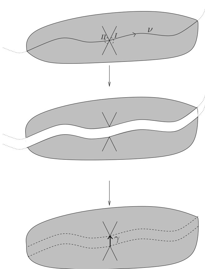
FIGURE 9. Breaking a zero of order two into two zeros of order one.
