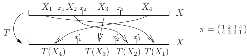
FIGURE 1. An interval exchange map and its corresponding permutation.
