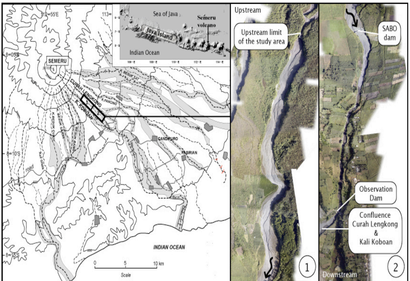
Fig. 1: Study area's location on Semeru volcano, East Java, Indonesia. The map shows the lahars inundation zone for the 20 th century largest events (Adapted from Thouret et al., 2007). The study area is limited upstream by a natural fall created by a lava deposit, and downstream the confluence between the Kali Koboan and the Curah Lengkok. At the observation dam, a French – Japanese collaboration set up a video camera system, and recently large sediments' traps.
