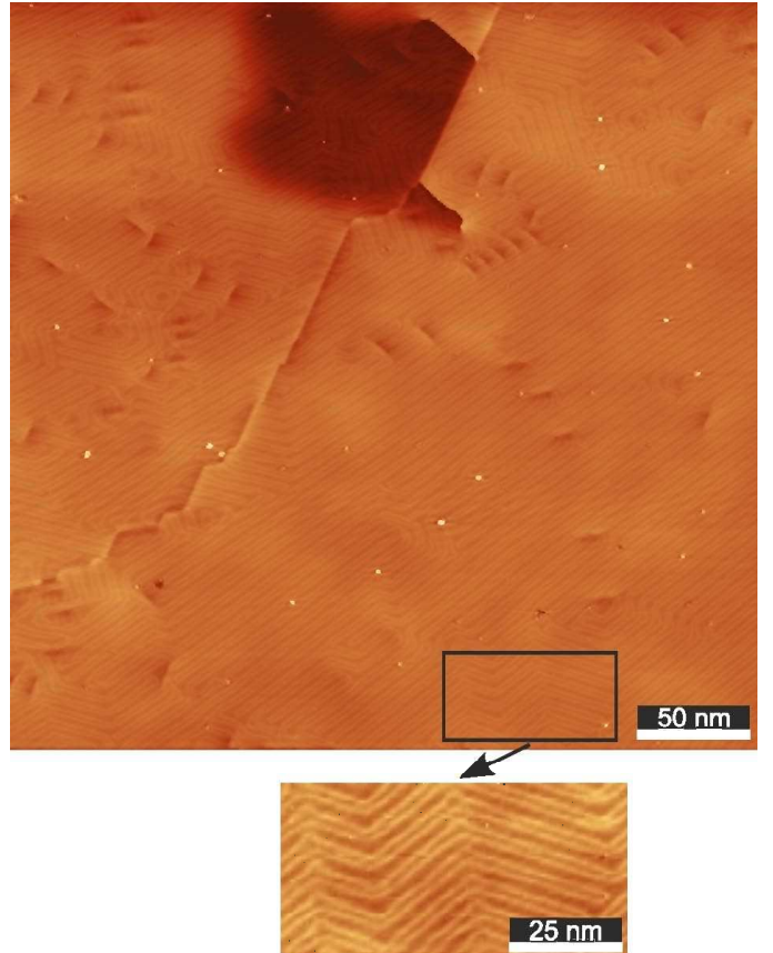
FIG. 1: (Color online) 375 \times 375 \text{ nm} STM image of Au(111) grown on Mo(110) (sample voltage 1 V, current 0.25 nA). The gray scale has been adjusted between zero and the maximum height Z_{max}=1.5 \text{ \AA} . A zoom of a selected area is shown in the lower part, displaying the Au(111) herringbone reconstruction with Z_{max}=0.54 \text{ \AA} .
