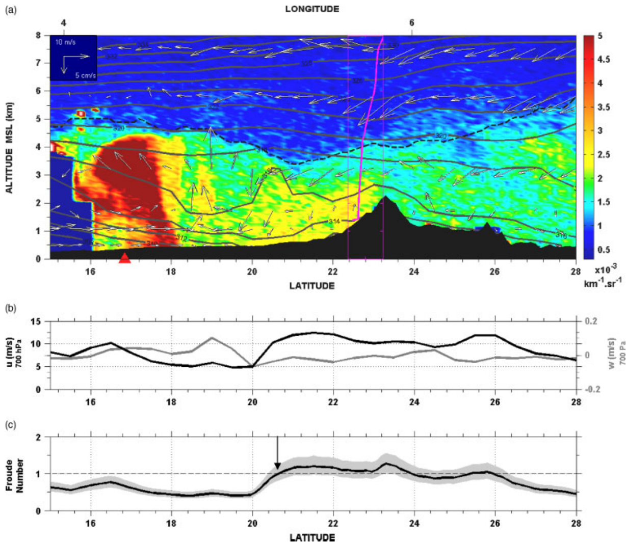
Figure 4. (a) Same as Figure 2(a), but on the 1 July 2006 at 01:37 UTC and arrows represent the flow along CALIPSO cross-section at 0000 UTC (i.e. ECMWF vertical and horizontal components projected along the satellite cross-section). The dashed black line is the SABL top. Tamanrasset virtual temperature profile from the 0000 UTC sounding is superimposed. (b) ECMWF analysis at 700 hPa of horizontal wind speed u (black) and vertical velocities w (gray). (c) Froude number in the SABL. The arrow indicates the hydraulic jump position.
