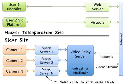
Fig. 3: Zoom on the streaming network architecture
