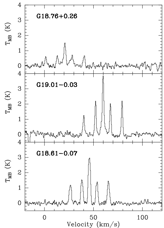
Fig. 7. Example spectra in \text{NH}_3 (1,1) transition for three sources located in the region shown in Fig. 6. G18.76+0.26 is probably at a distance of \sim 14 kpc, while G19.01-0.03 and G18.61-0.07 are probably at 4.3 and 3.7 kpc, respectively.
