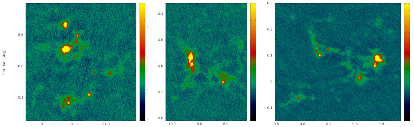
Fig. 4. Zooms into selected regions. These maps are projected with three pixels per beam, resulting in a pixel r.m.s. between 80 and 130 mJy/beam. All maps are shown in linear scale, calibrated to Jy/beam. The color scale has been chosen to highlight the negative artifacts, but doesn't cover the full range of fluxes in these images: the brightest peaks are, from left to right, 18.6, 17.2 and 7.2 Jy/beam; the most negative pixels are at -0.49, -0.54 and -0.43 Jy/beam, respectively.
