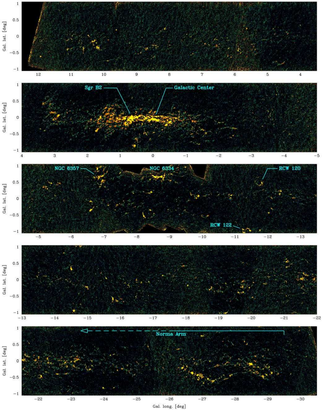
Fig. 3. Combined maps showing 84 deg 2 of the ATLASGAL data obtained in 2007, at 870 \mu\text{m} with a resolution of 19". The color scale is logarithmic between 0.05 and 1.0 Jy/beam. The rms is of order 50 to 70 mJy/beam in most parts of these maps. A few known regions are labeled in the maps. See also Fig. 4.
