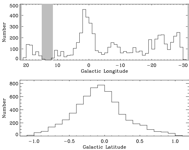
Fig. 5. Distribution of the 6000 compact sources in Galactic longitude (top, with 1^\circ bins) and latitude (bottom, with 0.1^\circ bins). Note that the longitude range +11.5^\circ to +15^\circ is not covered by the present data.
