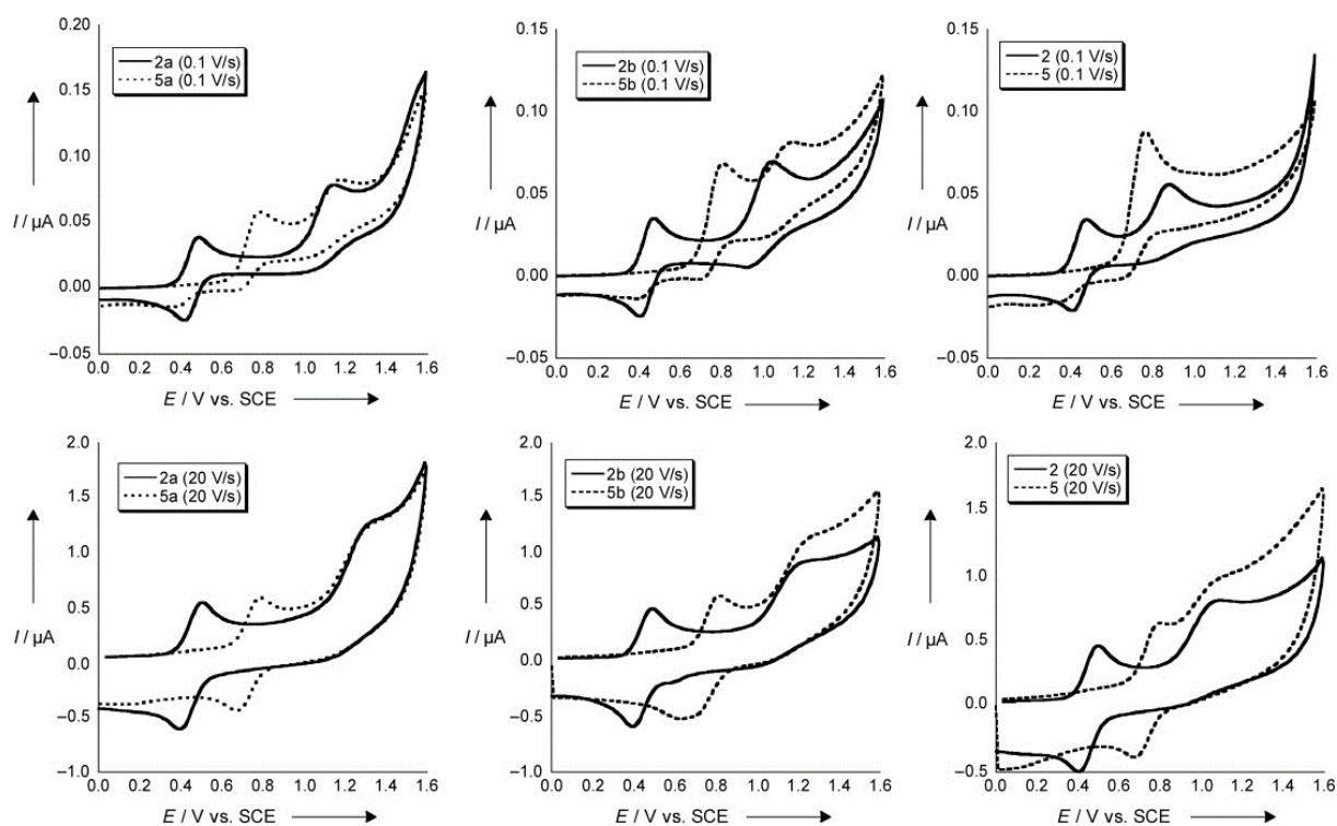
Figure 3 CVs of the alkylFc compounds (—) compared to their acylFc analogues (---) at low ( 0.1 \text{ V s}^{-1} ) and high ( 20 \text{ V s}^{-1} ) scan rates in DMF/0.1 M \text{Bu}_4\text{NBF}_4 .
