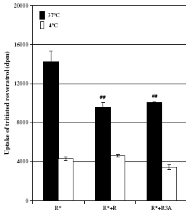
Fig. 3. Competitive effect of resveratrol or resveratrol triacetate excess on tritiated resveratrol uptake by HepG2 cells. HepG2 cells were incubated at 37 °C or at 4 °C for 10 min with [ 3 H] resveratrol alone in complete medium (R*) and with a 20-fold excess of resveratrol triacetate (R3A) or unlabeled resveratrol (R). After cell lysis, the cell-associated radioactivity was counted to determine tritiated resveratrol uptake. Presented data are from a representative experiment among three and each point represent the mean of three determinations on separate wells \pm SD. Values are significantly different by Mann–Whitney test from the control tritiated resveratrol uptake at 37 °C with p < 0.01 (##).
