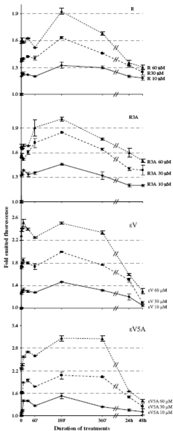
Fig. 5. Time course of HepG2 cells polyphenols uptake evaluated by fluorescence emission. HepG2 cells were treated with 0.1% ethanol (control), 10, 30 and 60 μM resveratrol (R), resveratrol triacetate (R3A), o-viniferin (oV) or o-viniferin pentacetate (oV5A) for 1, 2, 5, 10, 30 min, 3, 6, 24 and 48 h. After treatment, cells were harvested, quickly washed in cold PBS and maintained at 4 °C during flow cytometry analyses. Cells were excited by using a 350 nm lamp and the emitted fluorescence (>420 nm) was acquired in a FL4 channel. Values are means of the cell fluorescence fold increase from three different wells against controls of one representative experiment among three independent ones ±SD. All kinetics were significantly different from the control after ANOVA tests with p < 0.05 .
