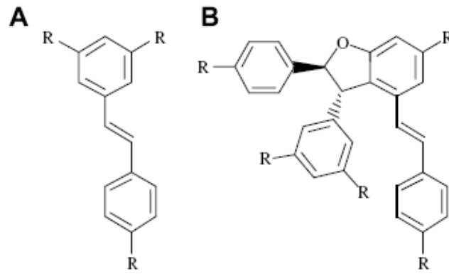
Fig. 1. Chemical structures of compounds. Chemical structures of trans -resveratrol (A, R=OH), trans -resveratrol triacetate (A, R=CH 3 -COO), \epsilon -viniferin (B, R=OH), and \epsilon -viniferin pentaacetate (B, R=CH 3 -COO).
