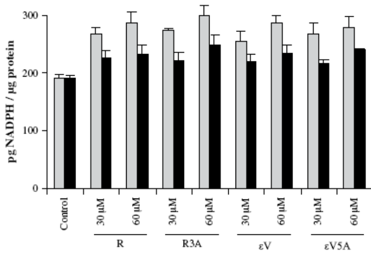
Fig. 6. Polyphenols induced NADPH accumulation. HepG2 cells were treated with 0.1% ethanol (control), 30 and 60 \mu\text{M} of resveratrol, resveratrol triacetate, \epsilon -viniferin and \epsilon -viniferin pentaacetate for 48 h. After 3 and 6 h, cells were lysed and NADPH amount in extracts were quantified. Values are means of NADPH levels in three different wells of one representative experiment among three independent ones \pm SD after 3 h or 6 h treatments \blacksquare . All NADPH levels in treated cells are significantly different from control cells and between 3 and 6 h treatments by Mann–Whitney test with p < 0.05 .
