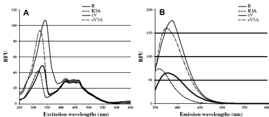
Fig. 4. Excitation (A) and emission (B) spectra of resveratrol (R), resveratrol triacetate (R3A), \epsilon -viniferin ( \epsilon V) and \epsilon -viniferin pentaacetate ( \epsilon V5A). Polyphenols stock solutions (10 \mu M) were prepared in ethanol and scanned in quartz microcuvets for fluorescence emission and excitation in a Kontron SFM25 spectrofluorimeter. Excitation spectra were obtained by all emitted wavelengths acquisition after excitation. Emission spectra were obtained by scanning emitted wavelengths at 330 nm light excitation. Ethanol spectra were used for baseline subtraction.
